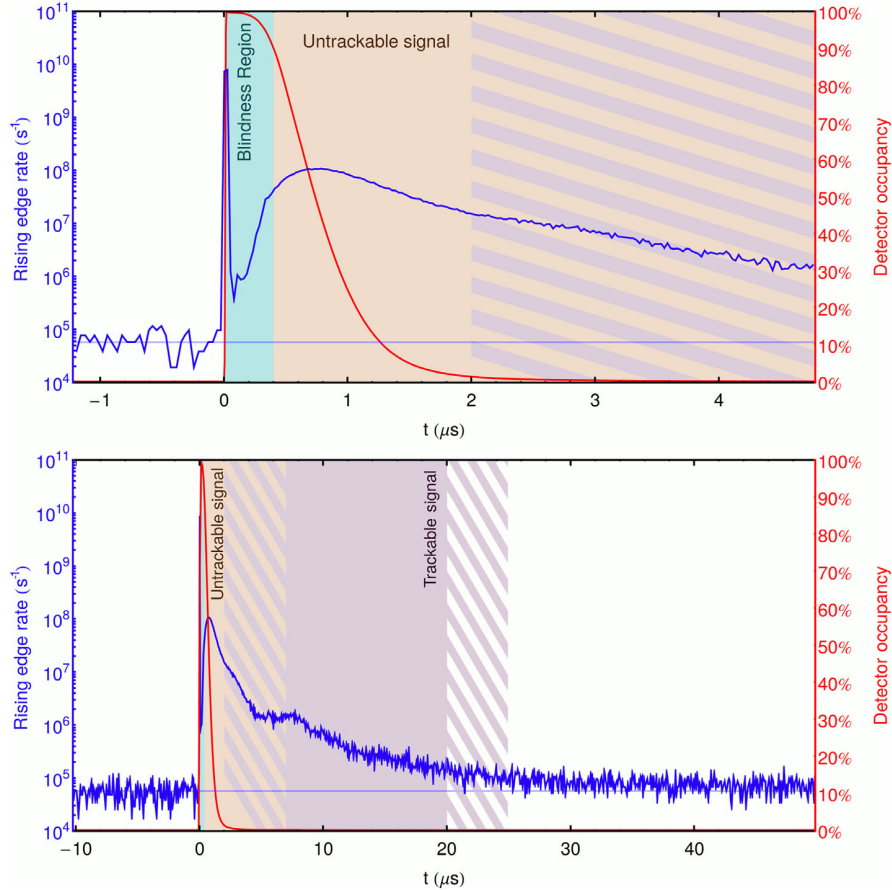
FIG. 17. Typical shape of the activity in FACT during an \bar{H} production cycle. The two frames show the same curve at different magnification levels. To obtain these profiles, 1027 different \bar{H} production cycles have been averaged together. The blue line shows the global rate of rising edges in the detector, the red curve which fraction of the detector’s fibers are above threshold at any single moment. The horizontal blue line indicates the dark count rate of 50\text{s}^{-1} per fiber. The first 0.4\ \mu\text{s} after the positron dump is a period of complete detector blindness. This period is followed (up to \sim 2\ \mu\text{s} ) by a partial recovery of the detector where fibers furthest away from the positron annihilation point exhibit periods of no activity while the central fibers are still on. This period consists fully of untrackable signal as shown in the upper panel of Fig. 18. Following this region, is a high activity region including a mix of untrackable and trackable signals (bi-colored hatched region). From \sim 7\ \mu\text{s} the signal is dominated by trackable signals as can be seen from the lower panel of Fig. 18. After \sim 20\ \mu\text{s} the signal becomes again a mix of untrackable and trackable signals (last hatched region in the lower panel) until the signal is consistent again with the average dark count rate of the detector. (For interpretation of the references to color in this figure legend, the reader is referred to the web version of this article.)
