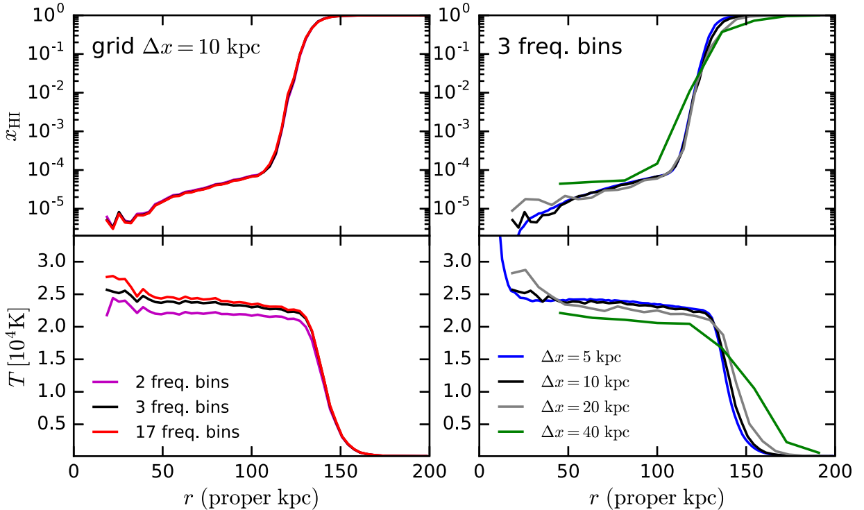
Figure A1. Numerical convergence test with the number of frequency bins below 54.4 eV and the size of the gas cells, for the case of a single ionizing source in an initially neutral homogeneous IGM. The source has a UV spectral slope of -1.5 and emits 5 \times 10^{52} ionizing photons \text{s}^{-1} . The top and bottom panels show the radial profiles of x_{\text{H I}} and T after evolving the gas for 10 Myr, respectively. Left: simulations have a grid size of 10 proper kpc and 2, 3, and 17 frequency bins. Right: simulations use three frequency bins, with grid sizes of 5, 10, 20, and 40 proper kpc. Overall, we find good numerical convergence with three frequency bins and cell sizes < 20 proper kpc, indicating that the IGM temperature in our simulations is well converged.
