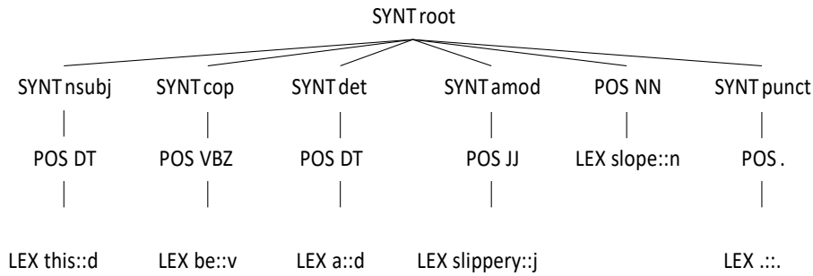
Figure 1: The GCRT representation for the sentence “This is a slippery slope.”
