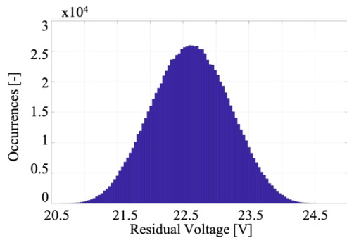
Fig. 7. PDF of |\bar{V}_R|_N for case #2
