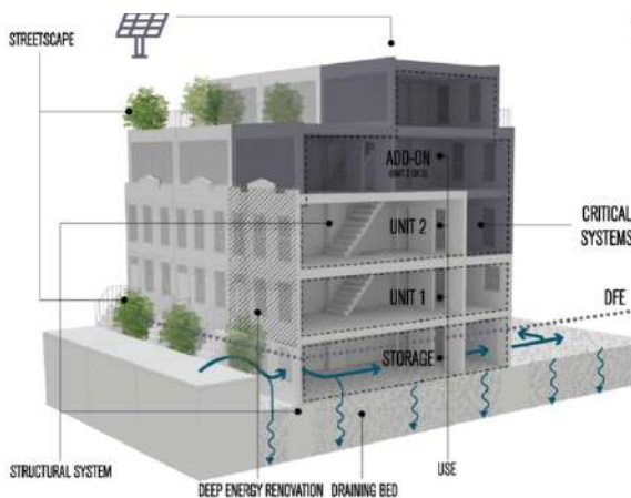
Figure 9. Deep Energy Renovation + Flood-Proofing + 2 Rooftop Add-ons in Pioneer Street
