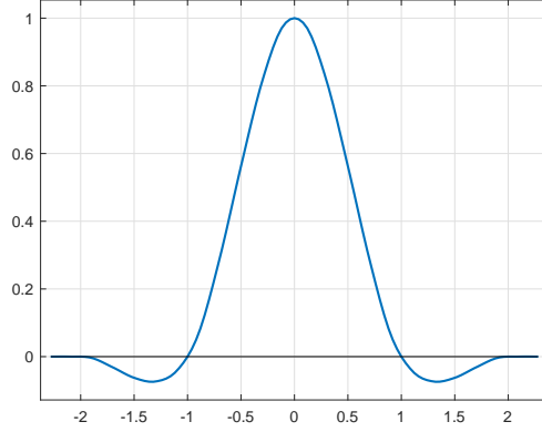
Figure 6: The basic limit function of the 5-ary scheme corresponding to the mask in (45) with w = -1.4 , which is supported in [-2.375, 2.375] , belongs to \mathcal{C}^{2.2044}(\mathbb{R}) and reproduces polynomials up to degree 2.
