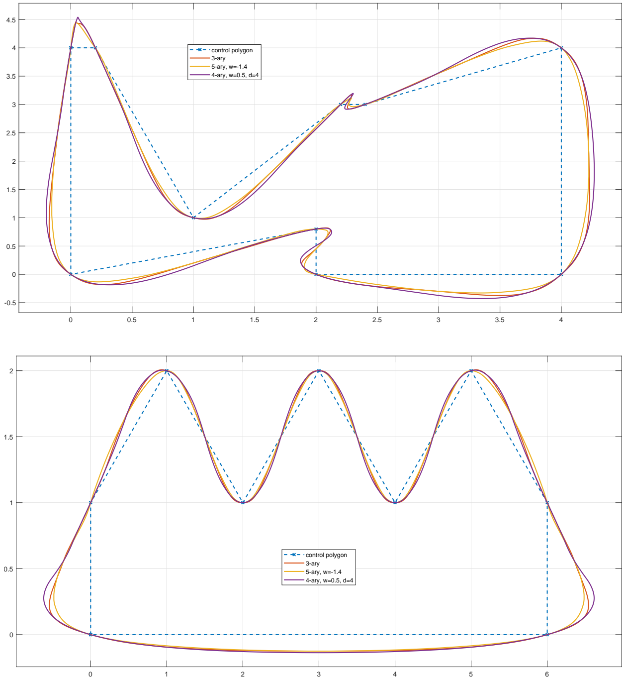
Figure 10: Comparison of the interpolations of polygons similar to the ones in [19] given by the schemes related to the masks (44), (45) with w = -1.4 and (47) with (48) and w = 0.5 .
