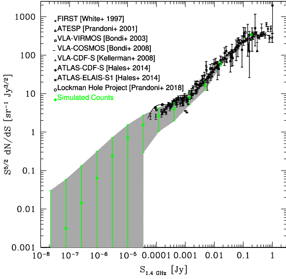
Figure 3. Euclidean-normalized source counts at 1.4 GHz: the black points represent the data (White et al. 1997; Prandoni et al. 2001; Bondi et al. 2003, 2008; Kellermann et al. 2008; Hales et al. 2014; Prandoni et al. 2018) while the green ones show the values obtained from the simulation of this work.
