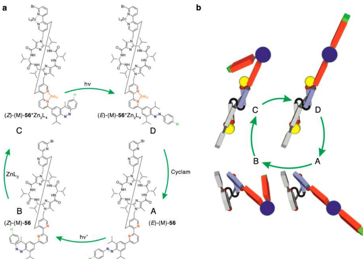
Figure 47. (a) Structural formula and operating cycle of four-stroke molecular motor 56. (b) Schematic representation of the different motor states. The bipyrindine unit bound to the azobenzene (red) pushing blade is colored light blue, and the other one is colored gray. The azo double bond is the dark-blue pivot, and the hydrogen atom that performs a 360° rotation during the operating cycle is highlighted in green. Adapted with permission from ref 358. Copyright 2011 Wiley-VCH Verlag GmbH & Co. KGaA, Weinheim.
