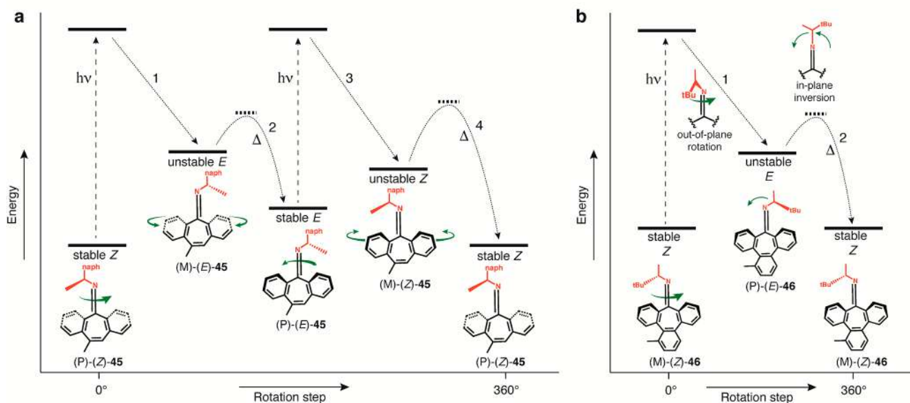
Figure 44. Structural formulas, operating mechanisms, and simplified energy profiles for 360° rotation of imine-based light-driven molecular rotary motors. 346 (a) Four-stroke motor 45 . Steps (1) and (3) denote E – Z photoisomerization, and steps (2) and (4) denote ring inversion. (b) Two-stroke motor 46 . Steps (1) and (2) denote E – Z photoisomerization and thermal nitrogen pyramidal inversion, respectively.
