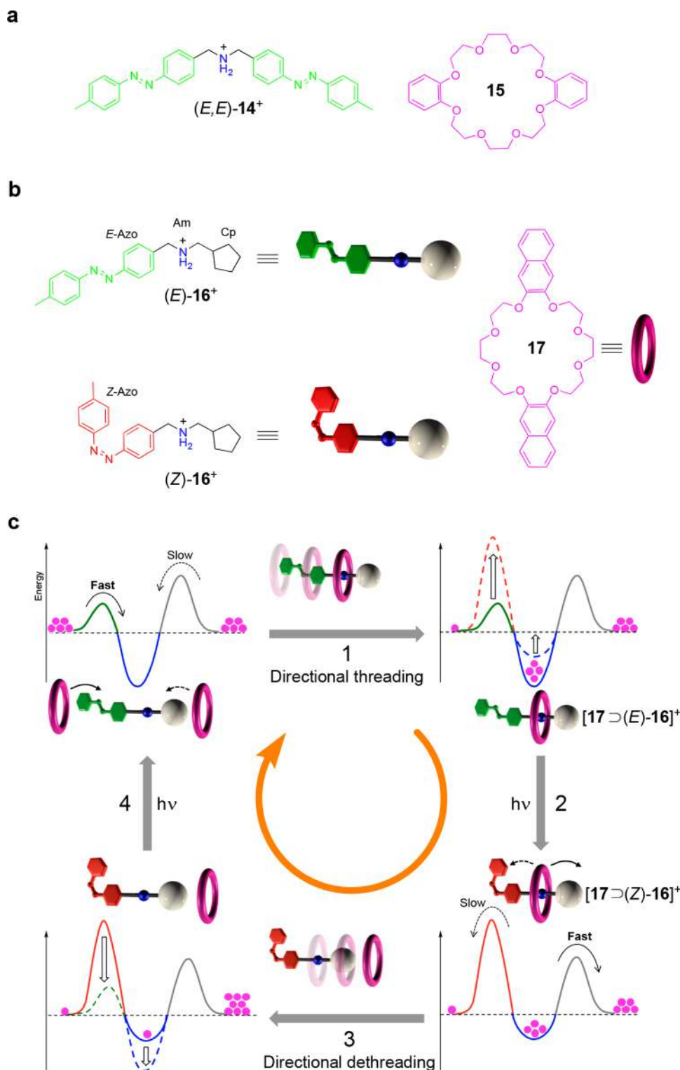
Figure 25. (a) Structural formulas of axle 14^+ in its E,E configuration and DB24C8 ring 15 . (b) Structural formulas and schematized representations of axle 16^+ in its E and Z configurations and ring 17 . (c) Schematic operation mechanism and simplified potential energy profiles, as functions of the ring–axle relative position, for each step (gray solid arrows) of the directional light-activated threading–dethreading motion (processes 1, 2, 3, and 4) of the ring and axle components. Dashed lines indicate processes that are kinetically prevented. The orange circular arrow shows the directional flux of species relevant in the operation of the system under steady-state out-of-equilibrium conditions. 291,293
