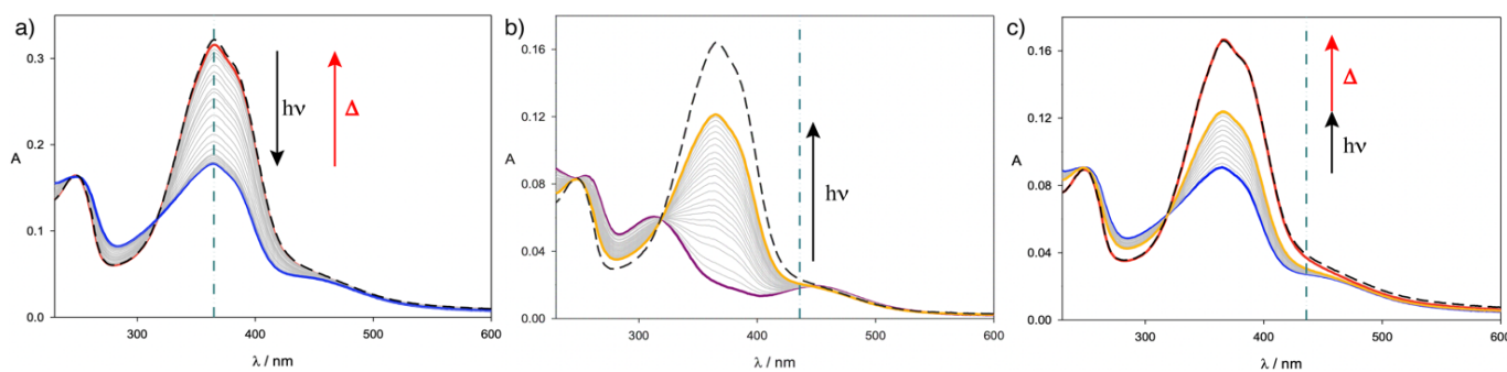
Figure 3. a) Absorption spectra of a spin coated film of E_4\text{-1a} before (black dashed trace) and after irradiation at 365 nm (blue trace); the red trace represents the spectra obtained after heating the irradiated film at 130 °C for 20 min. b) Absorption spectra of a spin coated film prepared from a solution of E_4\text{-1a} (black dashed trace) and from a solution of E_4\text{-1a} previously irradiated to the PSS with light of 365 nm before (magenta trace) and after exhaustive irradiation at 436 nm (orange trace). c) Absorption spectra of a spin coated film of E_4\text{-1a} (black dashed trace) and of a film of E_4\text{-1a} irradiated at 365 nm before (blue trace) and after irradiation at 436 nm (orange trace); the red trace represents the spectra obtained after heating the irradiated film at 130 °C for 20 min. Spectra taken at intermediate times during the irradiation are shown in light gray. The direction of the spectral variations of the \pi\pi^* band upon irradiation or heating are indicated respectively by black and red solid arrows. The vertical dashed lines mark the irradiation wavelength employed in the experiments.
