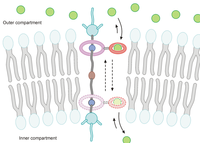
Figure 3. The transport of K + ions (green circles) across the lipid bilayer of a LUV through the thermally driven stochastic shuttling of a membrane-bound rotaxane (structure depicted in Figure 2).
