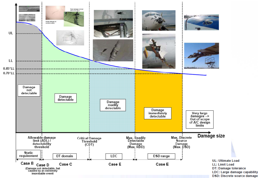
Figure 2: Load bearing capability based on impact damage size [3-4]
