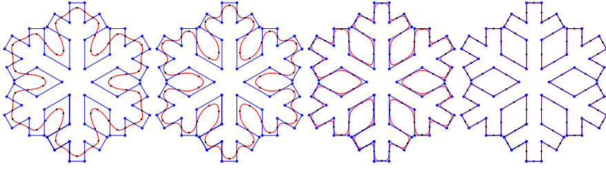
Fig. 10 C^5 splines, knot spacing h = 3 , all pieces taken from the space spanned by 1, \cosh(ax) \cos x, \cosh(ax) \sin x, \sinh(ax) \cos x, \sinh(ax) \sin x, \cosh(ax), \sinh(ax) . From left to right: a = 0.01; 0.7; 1.5; 3 .
