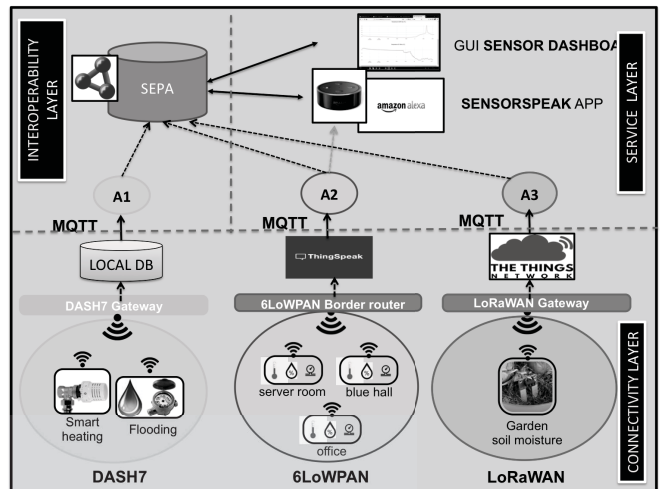
Fig. 2. The concrete IoT architecture currently implemented at ARCES@UNIBO
