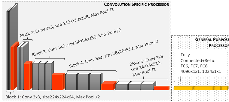
Fig. 8. VGG16 topology[34]. Gray layers indicate 3×3 convolutional layers; the Max Pooling reduction layers are in red, while the Fully Connected layers are in yellow. The two surrounding boxes highlight how the layers are mapped on the NEURAGHE platform.
