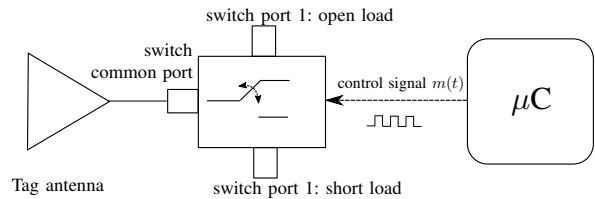
Fig. 3. Tag block schematic.
