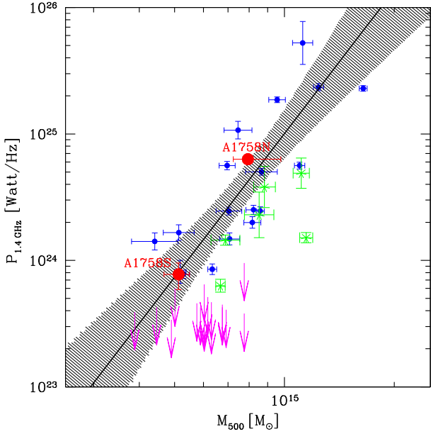
Figure 10. The P_{1.4}-M_{500} relation for giant radio haloes. Different colours indicate: giant radio haloes (blue), ultra-steep spectrum radio haloes (green), upper limits from Venturi et al. (2008) (magenta), and the radio haloes in A1758N and A1758S (red). Errors on P_{1.4} are smaller than the point size. The best-fitting relation for giant radio haloes and its 95 per cent confidence level are shown. Adapted from Cassano et al. (2013).
