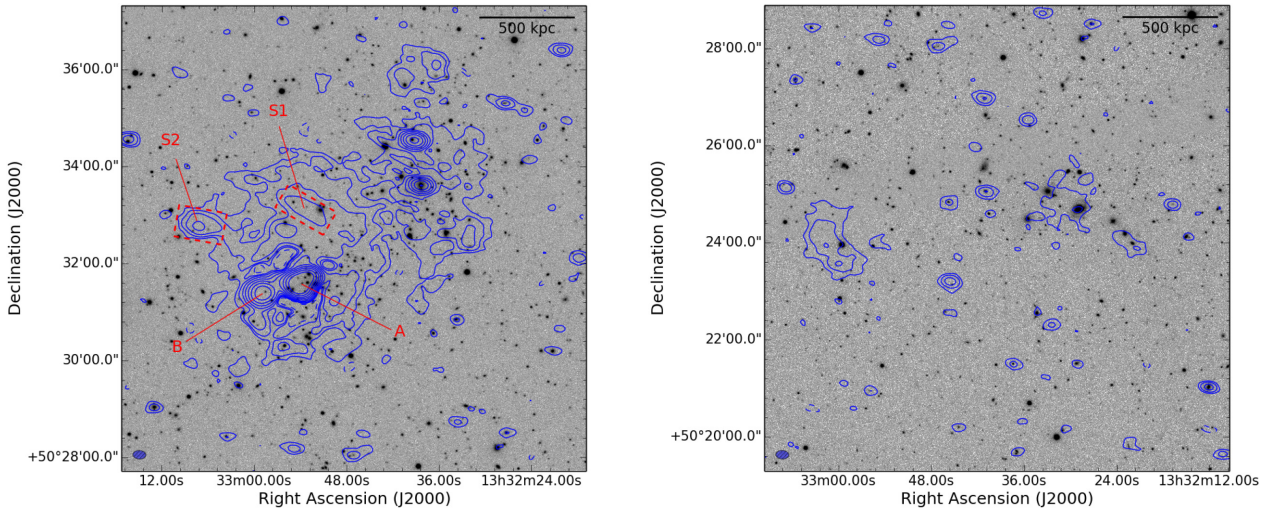
Figure 5. Mosaic SDSS g,r,i images of A1758N ( left ) and A1758S ( right ) overlaid with the LOFAR contours spaced by a factor of 2 starting from 3\sigma , where \sigma_{\text{LOFAR}} = 140 \mu\text{Jy beam}^{-1} . The negative -3\sigma contours are shown in dashed. The beam size is 16 \text{ arcsec} \times 11 \text{ arcsec} and is shown in the bottom left corners. At this resolution the radio halo in A1758S is marginally visible. More details on the LOFAR image are reported in Table 2.
