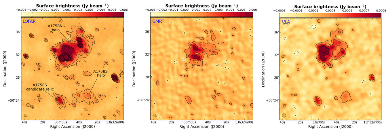
Figure 1. The cluster A1758 as observed in the radio band with LOFAR ( left ), GMRT ( centre ), and VLA ( right ). The point sources were subtracted in the GMRT and VLA images. Contours are spaced by a factor of 2 starting from 3\sigma , where \sigma_{\text{LOFAR}} = 230 \mu\text{Jy beam}^{-1} , \sigma_{\text{GMRT}} = 400 \mu\text{Jy beam}^{-1} , and \sigma_{\text{VLA}} = 70 \mu\text{Jy beam}^{-1} . The negative -3\sigma contours are shown in dashed. The beam sizes are 34 \text{ arcsec} \times 23 \text{ arcsec} (LOFAR), 43 \text{ arcsec} \times 29 \text{ arcsec} (GMRT), and 43 \text{ arcsec} \times 38 \text{ arcsec} (VLA) and are shown in the bottom left corners. More details on the images are reported in Table 2.
