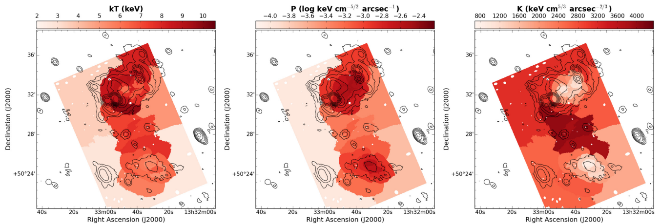
Figure 8. Thermodynamical properties of the ICM in A1758 with overlaid the LOFAR contours of Fig. 1. Images depict projected values of temperature ( left ), pressure ( centre ), and entropy ( right ). The temperature error map and a lower S/N temperature map are reported in Appendix A.
