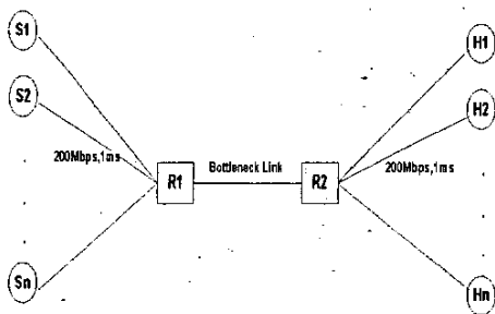
Figure 1. Network topology for simulations
