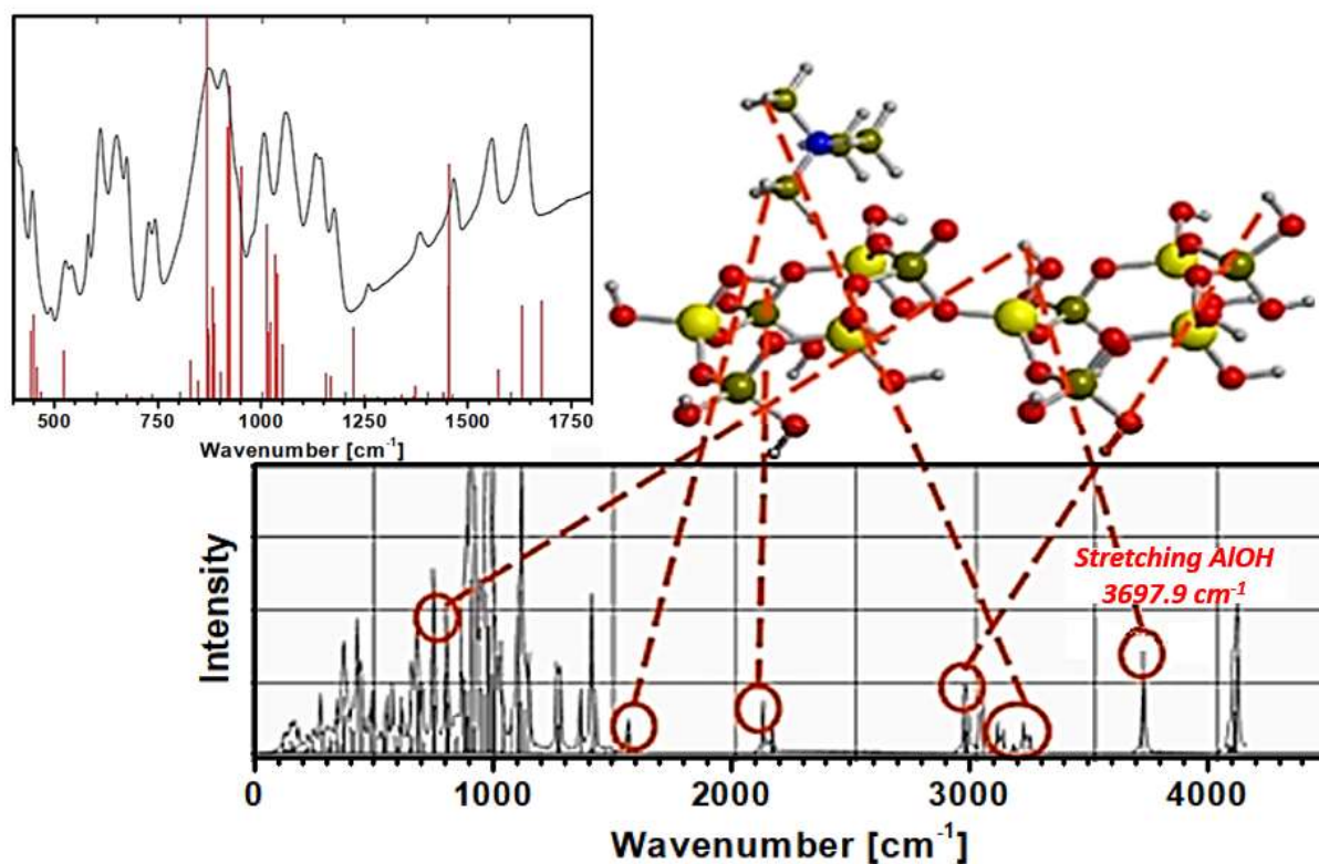
Fig. 14 Top: comparison of experimental (black) and DFT (red, 80 \text{cm}^{-1} shifted for anharmonicity) vibrational spectra of AlPO-butylammonium; Bottom: theoretical assignment of the main peaks in the simulated spectrum. Adapted with permission from ref. 175. Copyright 2008 American Chemical Society.
