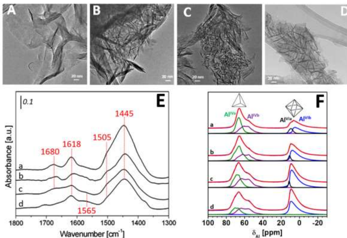
Fig. 10 top) TEM images of synthetic saponite samples prepared by using different H_2O/Si ratio (A: H_2O/Si=20 , B=50, C=110, D=150); bottom left) FT-IR spectra, in the 1800\text{--}1300\text{ cm}^{-1} region, of NH_3 (100 mbar) adsorbed and subsequently evacuated at r.t. on saponites prepared using H_2O/Si ratio of (a) 20, (b) 50, (c) 110 and (d) 150 materials outgassed at 573 K; bottom right) ^{27}Al MAS NMR data recoded using a MAS rate of 15 kHz, each spectrum includes experimental and deconvoluted spectra with individual contributions from each ^{27}Al site. Adapted with permission from ref. 131. Copyright 2012 Elsevier Ltd.
