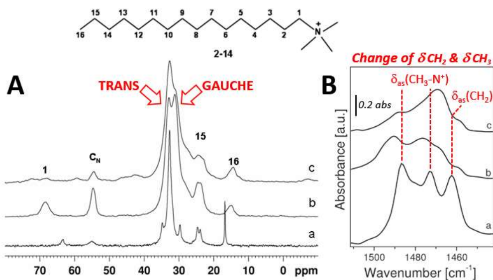
Fig. 11 (A) ^{13}\text{C} CPMAS NMR spectra of: pure CTABr (a), CTA-SAP_PS (b) and CTA-SAP_OP (c); (B) IR spectra of CTABr (a), CTA-SAP_PS (b) and CTA-SAP_OP (c) samples diluted in KBr. \text{C}_\text{N} denotes methyl carbons directly bound to nitrogen. Adapted with permission from ref. 111. Copyright 2011 American Chemical Society.
