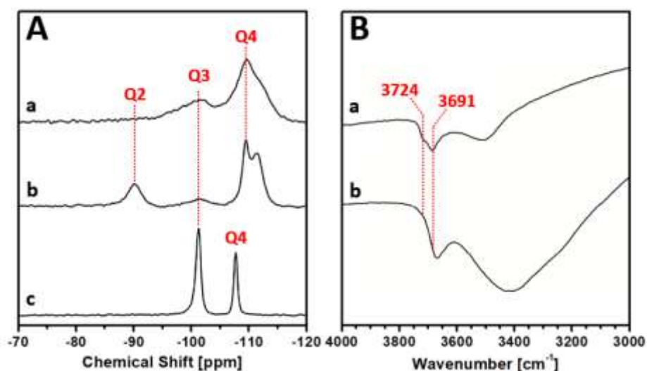
Fig. 18 (A) ^{29}\text{Si} MAS NMR spectra of (a) RUB-51, (b) Tetra-RUB-51, and (c) Heated-Tetra-RUB-51 and (B) IR spectra of (a) Heated-Tetra-RUB-51 and (b) Heated-Tetra-RUB-51 after heating at 200 ^{\circ}\text{C} for 4 h. Adapted with permission from ref. 273. Copyright 2014 American Chemical Society.
