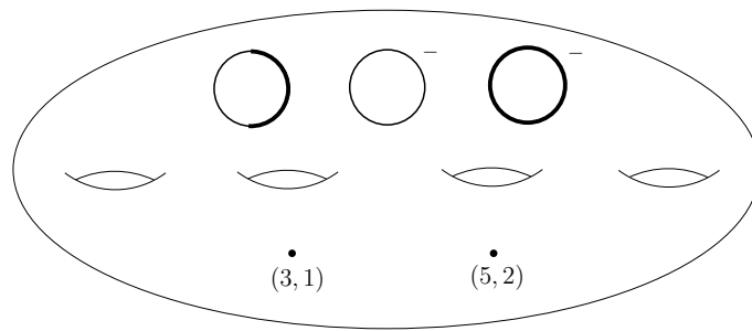
Figure 5: The Seifert fibre space \{0; (o, 4, (1, 1)); (1 | 0); ((3, 1), (5, 2))\} .
