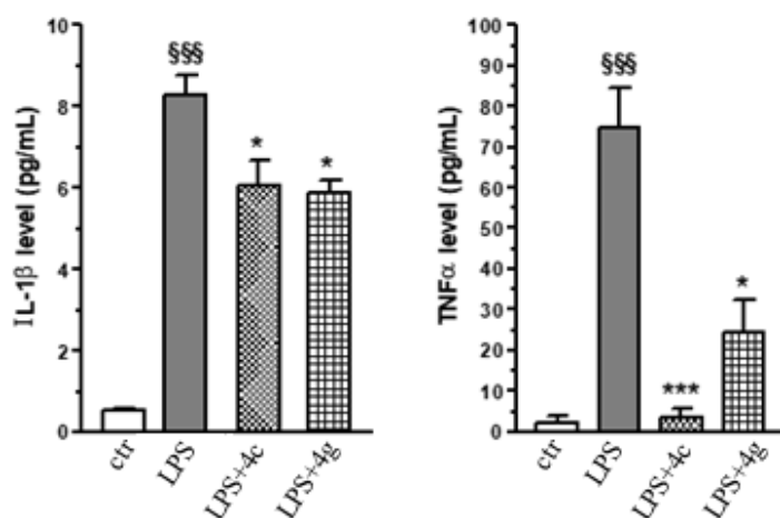
Fig. 12. Compounds 4c and 4g inhibit the release of TNF \alpha and IL-1 \beta induced by LPS in THP-1 cells, representative of human microglial cells. THP-1 cells were treated with compounds (10 \mu M) and LPS (1 \mu g/mL) for 24 h. At the end of the treatment, the pro-inflammatory cytokine levels were determined as described in the experimental section. The values are reported as mean \pm SD of three independent experiments. §§§ p < 0.001 vs. untreated cells, * p < 0.05 and *** p < 0.001 vs. cells treated with LPS (ANOVA with Bonferroni post hoc test).
