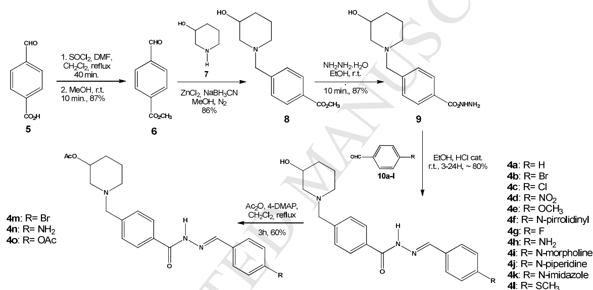
Scheme 1. Synthetic route for the target-compounds 4a-o
