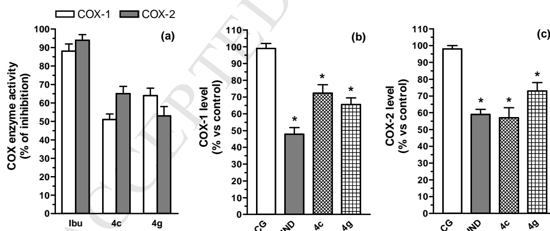
Fig. 8. Effect of compounds 4c and 4g on COX-1 and COX-2 enzyme activity and blood levels. (a) In vitro peroxidative activity of human COX-1 and ovine COX-2 was determined by a chemiluminescence assay in the presence of compounds (10 \mu M) or ibuprofen (Ibu), as a positive control. Values are the mean \pm SEM of two independent experiments. (b, c) Plasma COX-1 and
