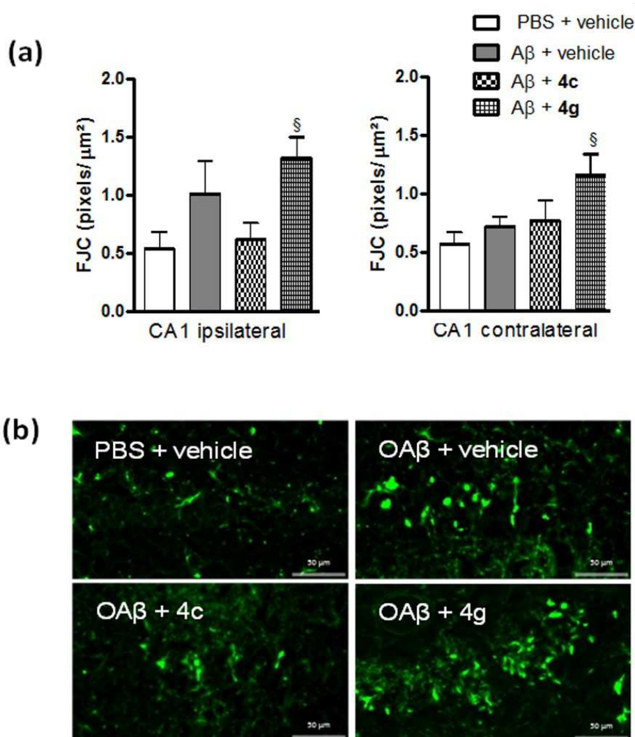
Fig. 15. Compounds 4c , but not 4g , counteract the neuronal death induced by unilateral intrahippocampal injection of A \beta_{1-42} O in mice. (a) The quantitative analysis of neuronal death in the CA1 area of the ipsilateral and contralateral hippocampus by FJC staining was performed 7 days after the administration of the compounds (100 mg/kg, i.p.) and A \beta_{1-42} O intrahippocampal injection in mice as reported in experimental section. (b) Representative FJC staining of hippocampus slices. Scale bar 50 \mu\text{m} . Values are expressed as mean \pm SEM ( n=10 ) of the pixel intensity of each hippocampus slice analyzed. ^{\S}p < 0.05 vs. PBS + vehicle; ^*p < 0.05 vs. A \beta O + vehicle; ANOVA, with Newman-Keuls post hoc test.
