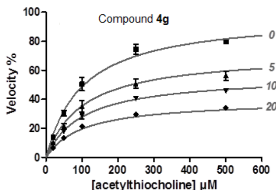
Fig. 3. Substrate competition assay of compound 4g for EeAChE. Data points are mean \pm SD from 3 independent experiments, each performed in triplicate. The curves represent the best-fitting noncompetitive inhibition model, with estimated parameters (and 95% C.I.): K_m = 101.9 (87.7 to 116.2) \mu\text{M} and K_i = 13.41 (11.87 to 14.96) \mu\text{M} . The inhibitor concentrations ( \mu\text{M} ) are indicated to the right of the curves.
