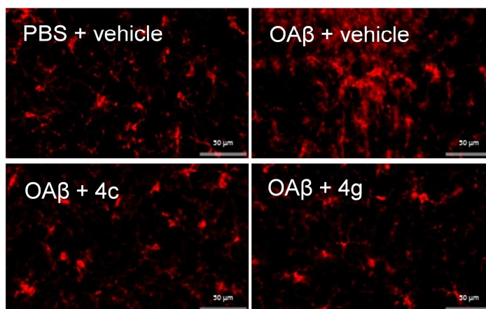
Fig. 13. Compounds 4c and 4g inhibit microgliosis induced by unilateral intrahippocampal injection of A \beta_{1-42} O in mice. (a) The quantitative analysis of microgliosis in the CA1 area of the ipsilateral and contralateral hippocampus by Iba1 immunostaining was performed 7 days after the administration of compound (100 mg/kg, i.p.) and A \beta_{1-42} O intrahippocampal injection in mice as reported in the experimental section. (b) Representative Iba1 immunostaining of the hippocampus. Scale bar 50 \mu m. Values are expressed as mean \pm SEM (n = 10) of the pixel density of each image analyzed. §§ p < 0.01 vs. PBS + vehicle; * p < 0.05 and ** p < 0.01 vs. A \beta + vehicle; ANOVA, with Newman-Keuls post hoc test.
