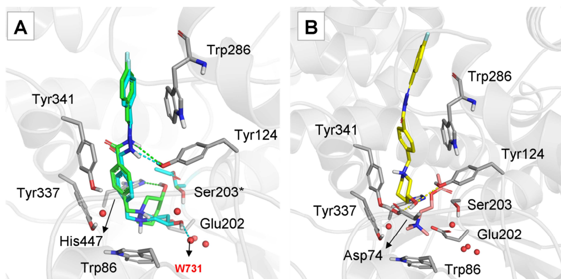
Fig. 4. Docking results for 4gR in the (A) free (green) and acetylated (light blue) states, and in the Michaelis complex (yellow). ACh is represented as salmon sticks and molecular waters as red spheres.
