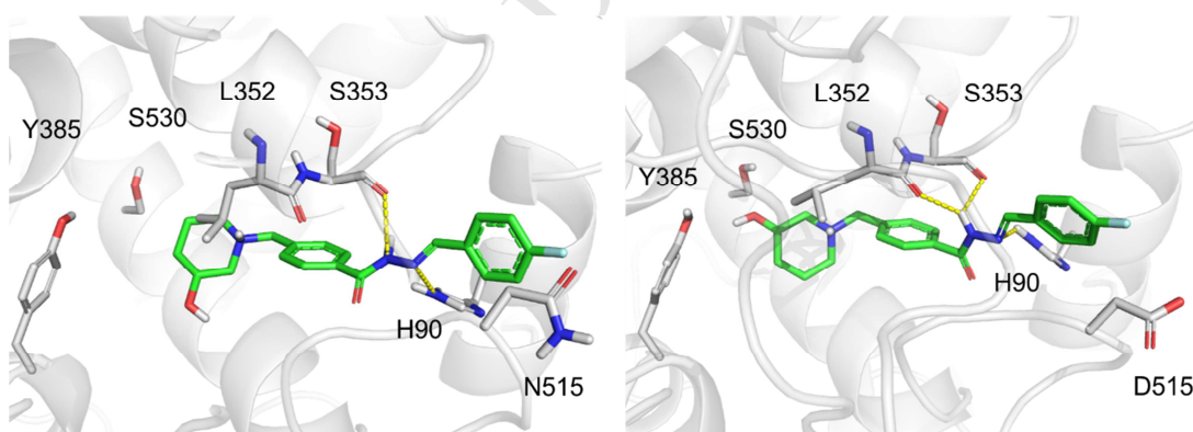
Fig. 11. Docking results of 4g (light green) in the COX-1 (left) and COX-2 (right) catalytic channels. Hydrogen bonds are represented as yellow dashes.
