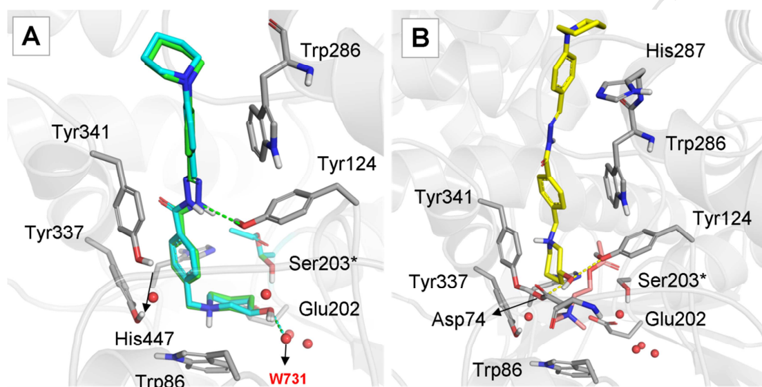
Fig. 6. Docking results for 4jR in the (A) free (green) and acetylated (light blue) states, and in the Michaelis complex (B, yellow). ACh is represented as salmon sticks and water molecules as red spheres.
