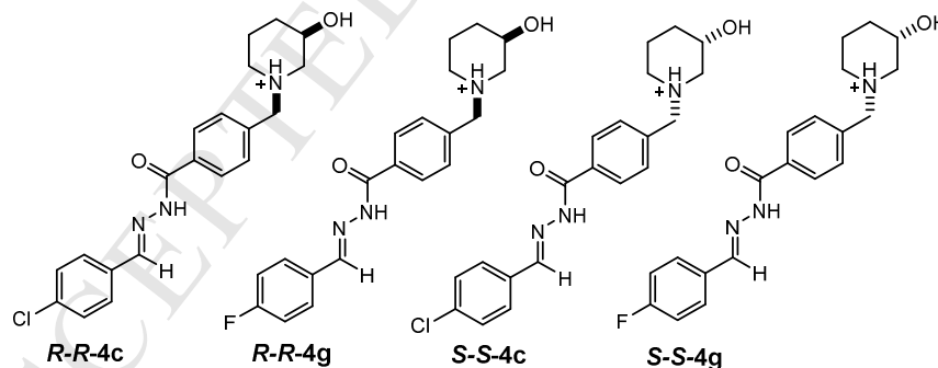
Fig. 9. 2D structures of ( R-R ) and ( S-S ) configurations of 4c and 4g .
