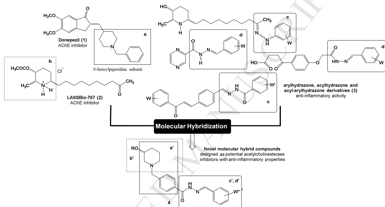
Fig. 1. Design of a new series (4) of multi-target directed ligands (MTDLs) based on the molecular hybridization of the structures of donepezil (1), the AChE inhibitor LASSBio-767 (2) and a series of anti-inflammatory N -aryl-acylhydrazone derivatives (3).
