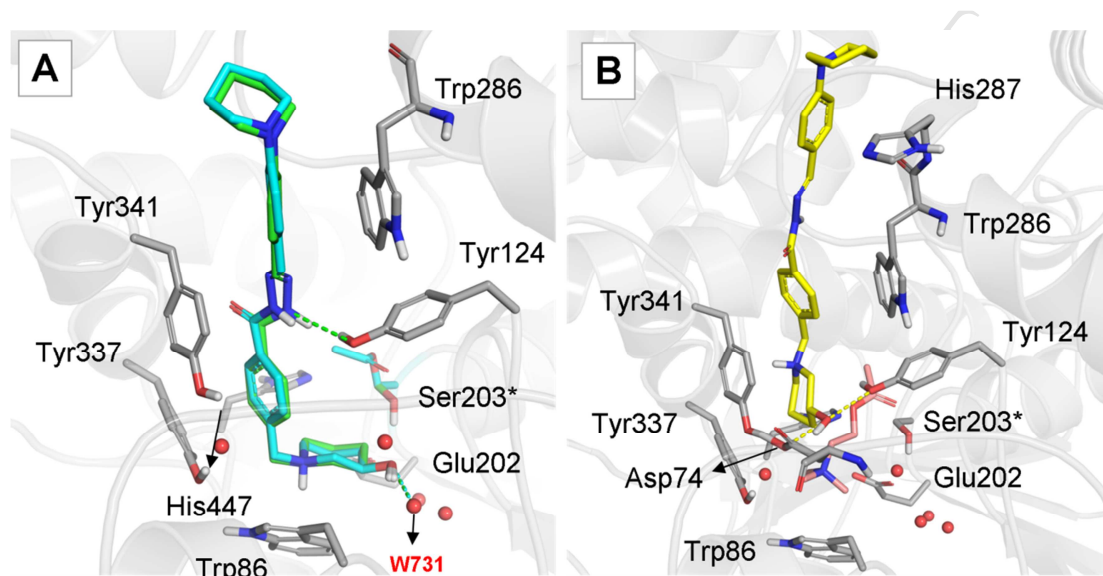
Fig. 6. Docking results for 4jR in the (A) free (green) and acetylated (light blue) states, and in the Michaelis complex (B, yellow). ACh is represented as salmon sticks and water molecules as red spheres.
