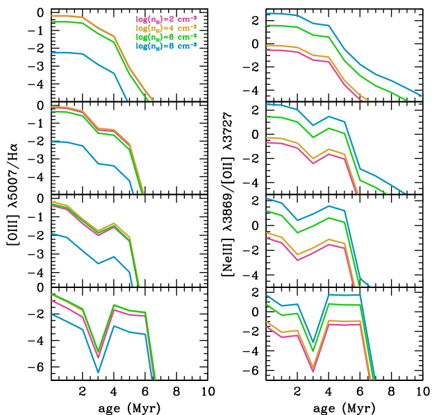
Figure 9. [O III]/H \alpha and [Ne III]/[O II] time evolution for different values of n_H , and \log(U)_0 = -3 . The hydrogen density increases from \log(n_H)=2 (which is our default value) to \log(n_H)=8 , from pink to cyan, as labelled. Metallicity ( Z = 0.004, 0.008, 0.02 and 0.04 ) increases from the top to the bottom panel.
