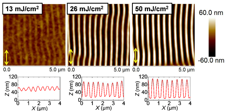
Figure 2. AFM height images of LIPSS on P3HT thin films created with 3600 pulses varying the fluence. Laser irradiation wavelength \lambda = 532 nm. Height profiles over lengths of 4 μm are shown at the bottom of the images. The double arrows indicate the polarization vector of the laser beam.
