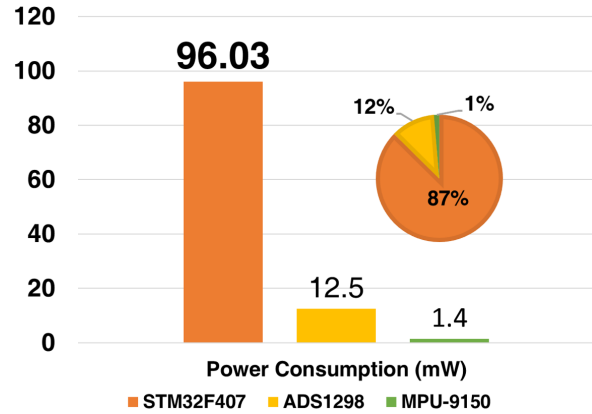
Figure 9: Power consumption of the embedded implementation (on PCB). The MCU dominates the power consumption, employing 87% of the total power.
