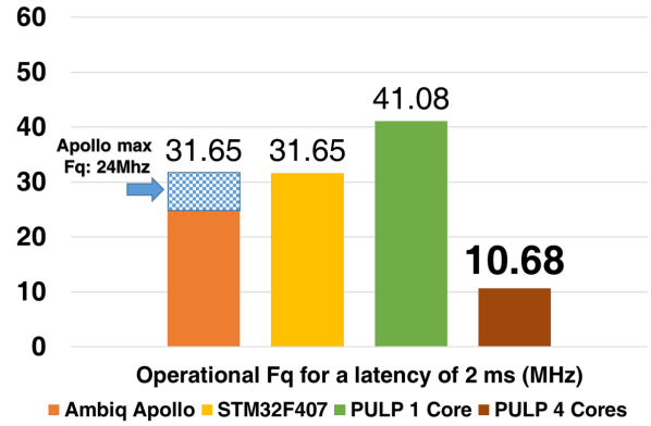
Figure 11: Minimal operating frequency required to achieve real-time operation. Featuring parallelization, the 4-cores PULP implementation is capable to work at a considerable lower frequency than the other cores, favoring voltage scaling and hence energy saving.
