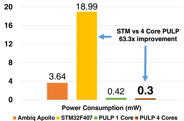
Figure 12: Power consumption comparison between different platforms. The 4-cores PULP MCU offers 63x energy saving with respect to the implementation on STM32F407.
