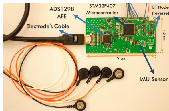
Figure 5: Assembled PCB (top) with electrodes cable. Here, two channels and the reference (GND) are wired. Only one channel (and reference) are later attached to the auto-adhesive gel-based electrodes to perform the tests.
