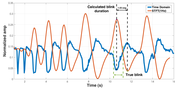
Figure 2: Blinks in time and frequency domain. The blue line represents the original EEG signal contaminated with the eye-blink artifacts (depressions of the signal) while the red line represents the energy values of the 1 Hz signals over time, extracted using the STFT.
