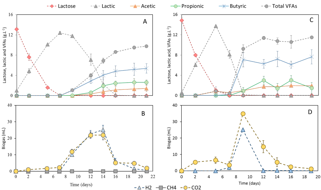
Figure 2: AFMC of CW at microcosm scale. Lactose, lactic acid, VFAs concentrations and biogas production trends for free suspended (A and B) and immobilized (C and D) cells conditions.
