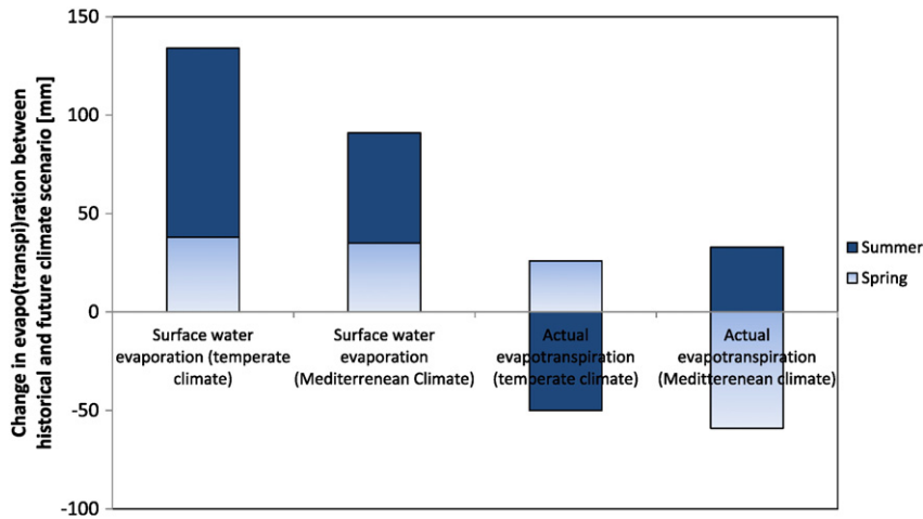
Fig. 12. Histogram showing the change in E and ETa for temperate and Mediterranean climate calculated with historical data and with a climate change scenario for the end of the century. A positive change means that the evaporation rate will increase.
