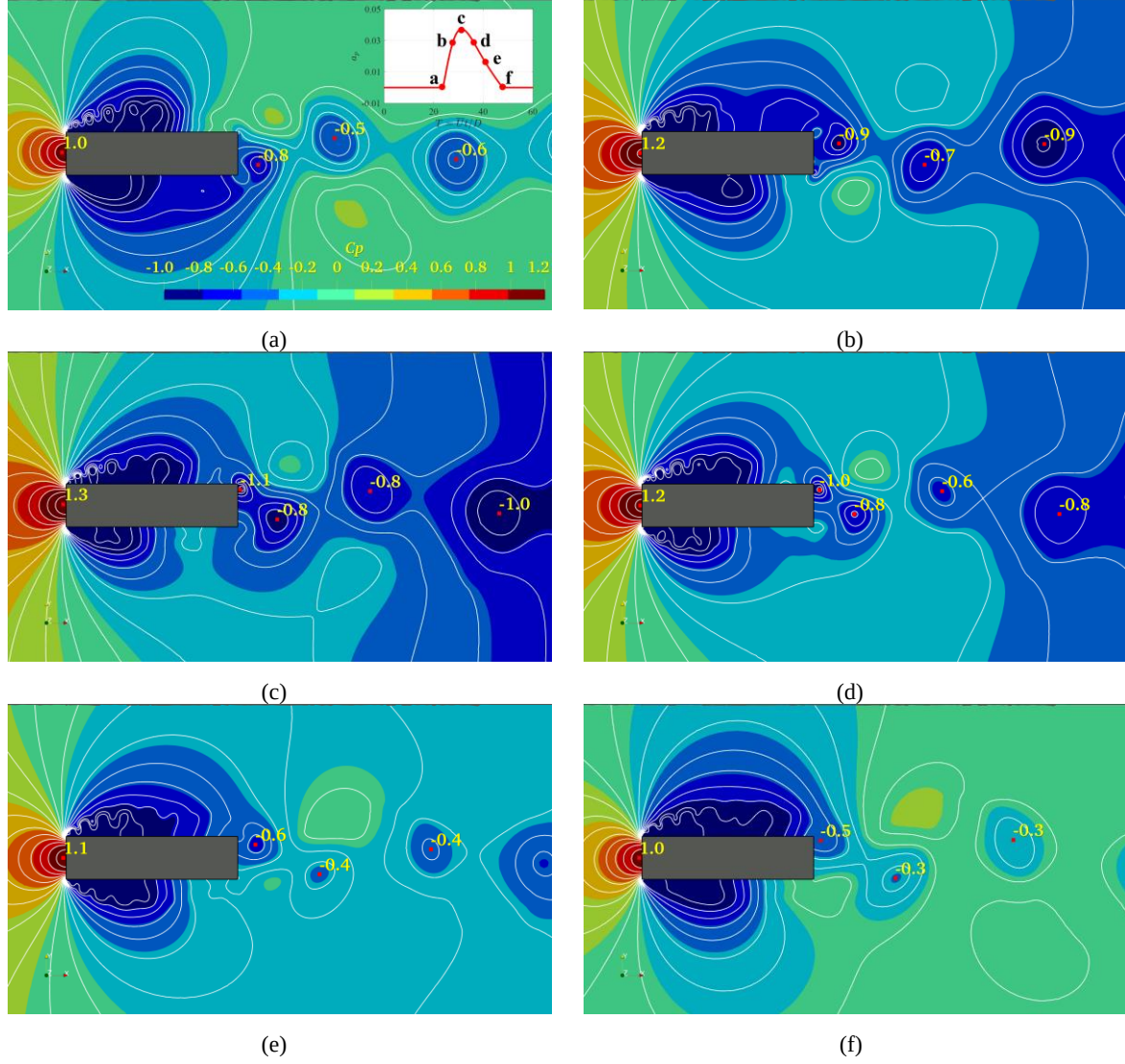
Figure 16. Pressure flow fields for R4 under S-3 conditions at different time instants: (a) T=24 ; (b) T=27.6864 ; (c) T=31.3752 ; (d) T=36 ; (e) T=40.8 ; (f) T=48 .
