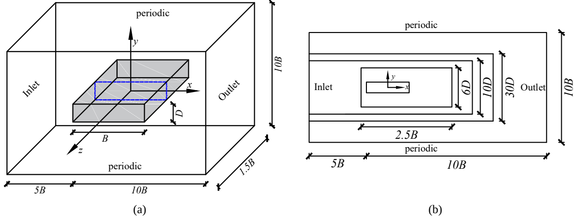
Figure 2. Numerical model: (a) computational domain; (b) mesh zones (the figure does not respect real proportions).
