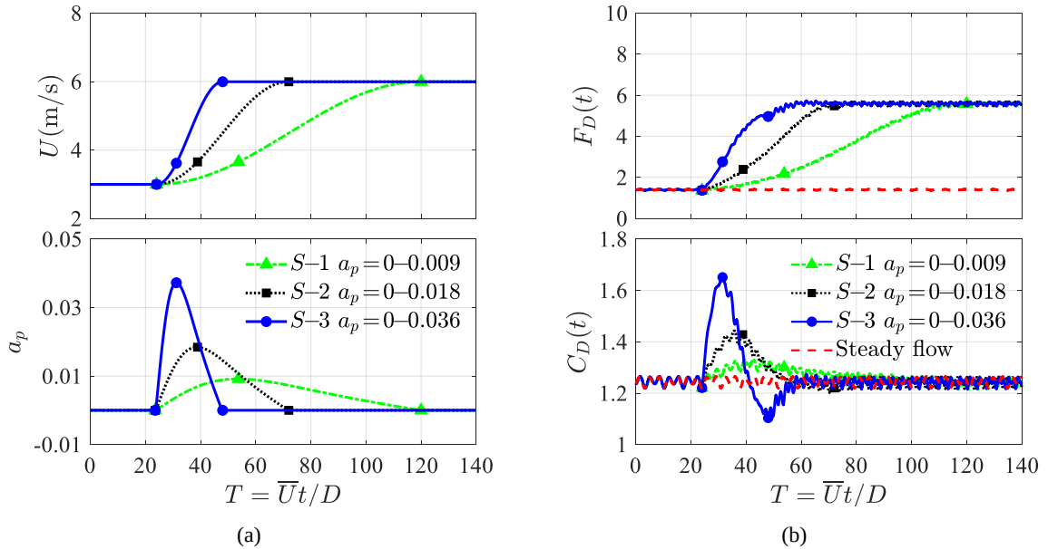
Figure 12. Drag coefficients of R4 for Sinusoidal -type accelerating flows: (a) U and a_p ; (b) F_D(t) and C_D(t) .
