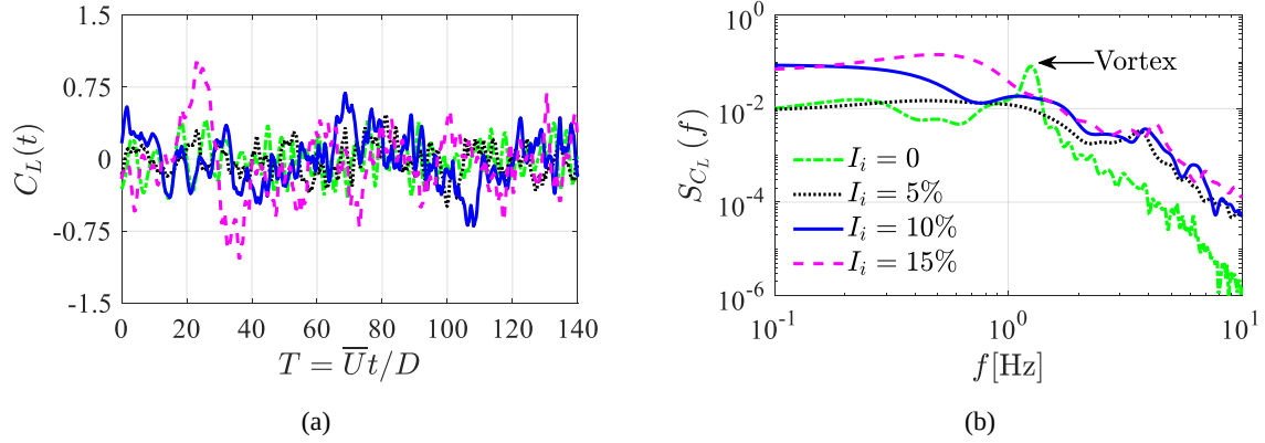
Figure 19 Lift coefficients from LES under Turbulent -type accelerating inflows with varying turbulence intensities: (a) time history; (b) spectrum.
