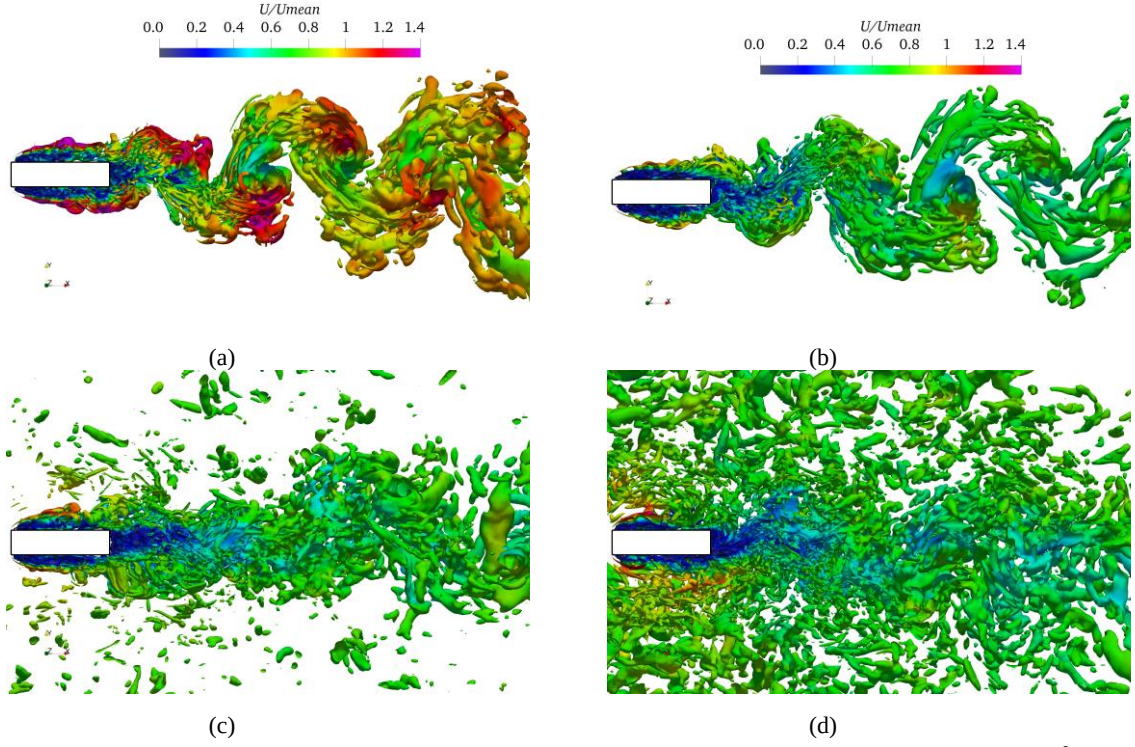
Figure 20 Q criterion of the instantaneous coherent structure for different turbulence intensity( Q=0.50 \text{ s}^{-2} ): (a) Steady flow (b) I_t=0 ; (c) I_t=5\% ; (d) I_t=10\% .
