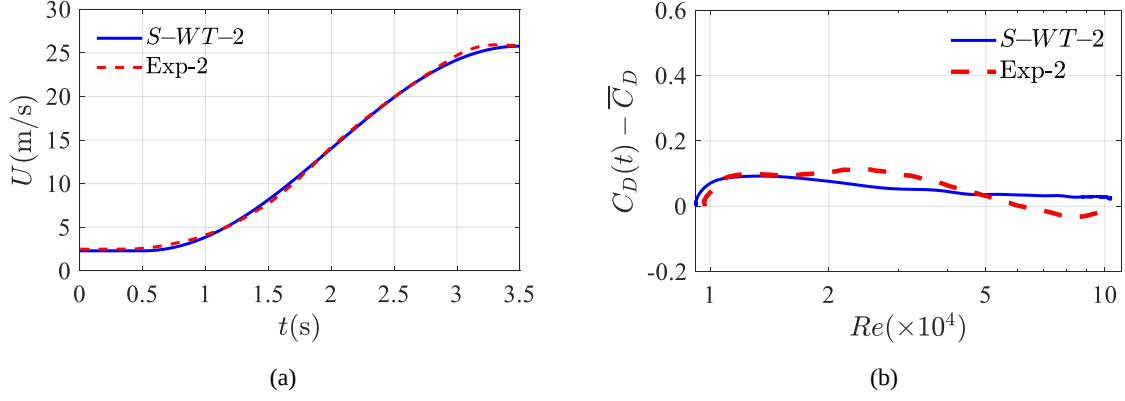
Figure 7. Time-varying drag coefficients of R3 for acceleration case S-WT-2 : (a) U ; (b) C_D(t) - \bar{C}_D .
