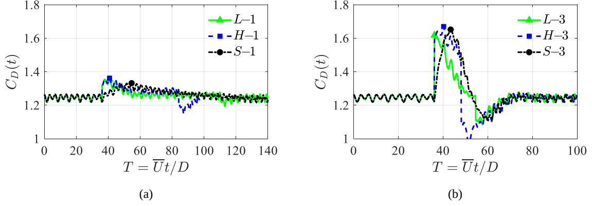
Figure 13. Drag coefficient of R4 under different accelerating flows with a_{p,max} of: (a) 0.009 and (b) 0.036.
