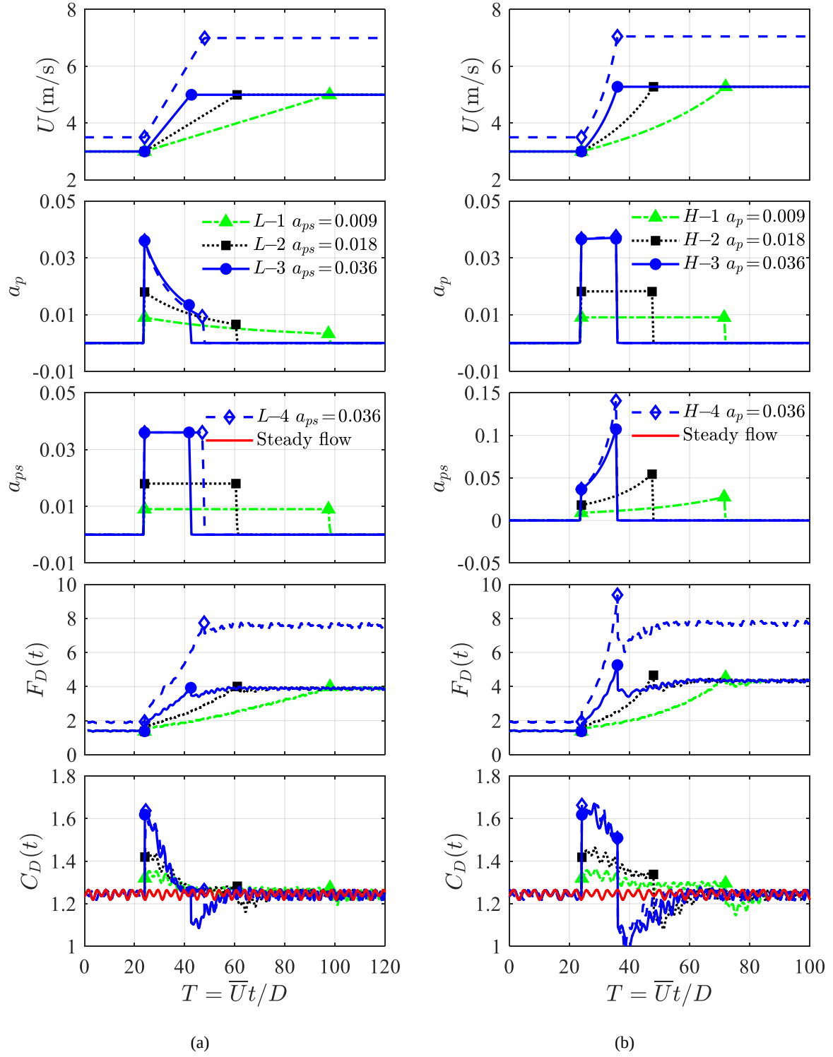
Figure 11. Drag coefficient of R4 for different accelerating flows: (a) Linear type; (b) Hyperbolic type.
