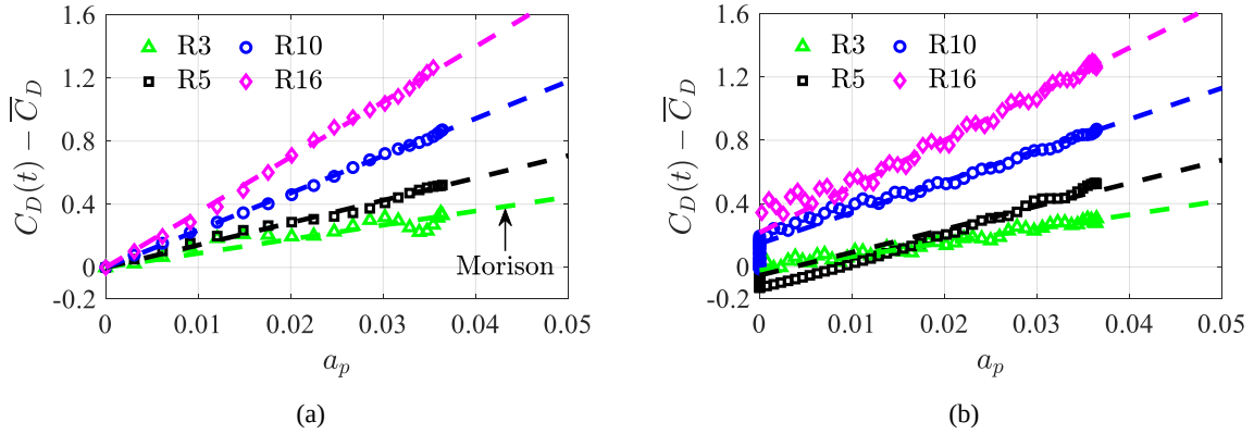
Figure 22. Drag coefficients vs accelerate parameter a_p for different rectangular cylinders: (a) a_p ramp-up phase; (b) a_p ramp-down phase.
