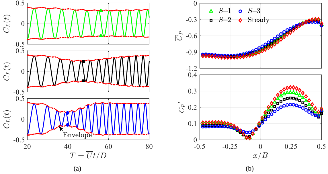
Figure 17. Lift Statistics of R4 in different Sinusoidal -type inflows: (a) time history of lift coefficients; (b) mean and stand deviation of pressure distributions during acceleration.
