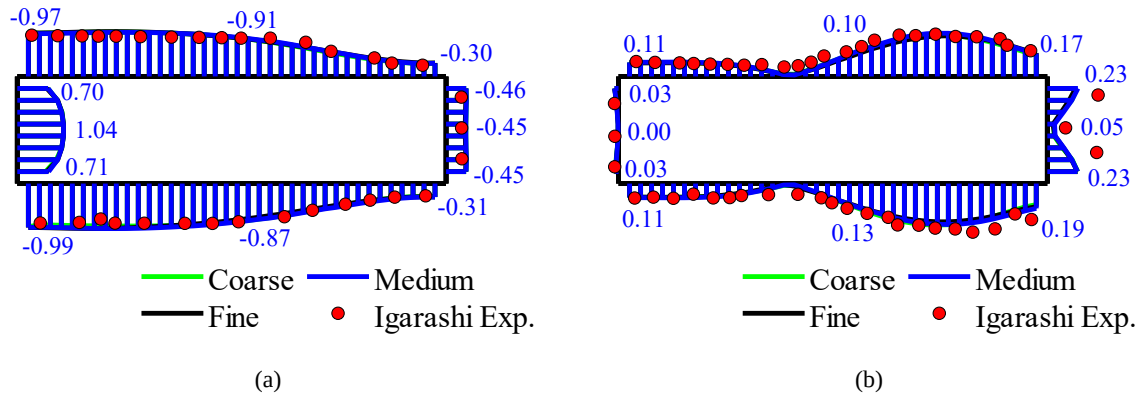
Figure 4. Pressure coefficients for R4 using URANS: (a) time-average; (b) standard deviation.
