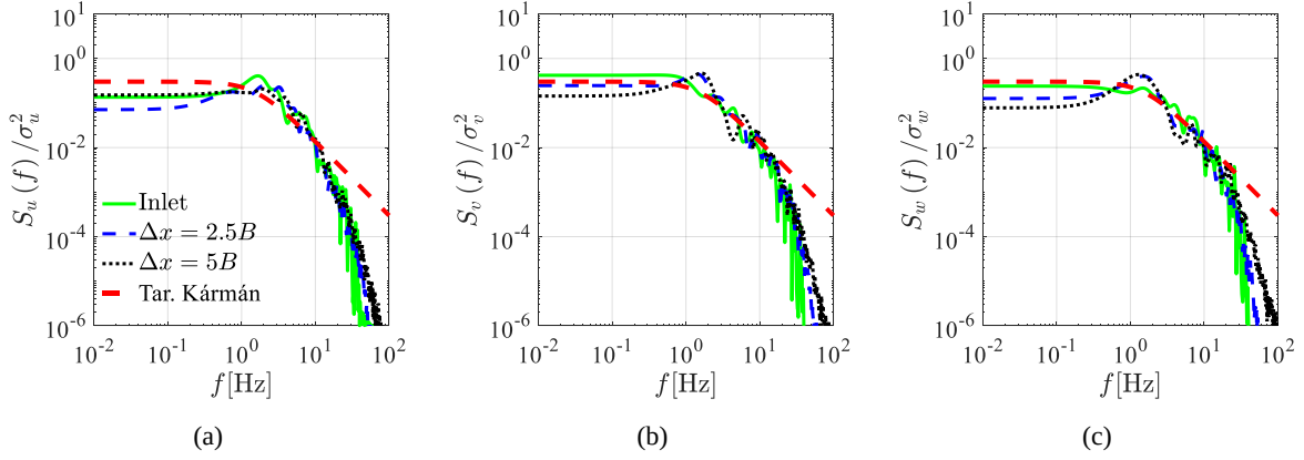
Figure 10. Spectra of fluctuating components of Turbulent -type accelerating inflow: (a) u ; (b) v ; (c) w .
