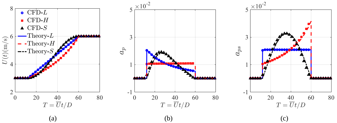
Figure 8. Comparison of three types of accelerating inflows wind fields: (a) U(t) ; (b) a_p ; (c) a_{ps} .
