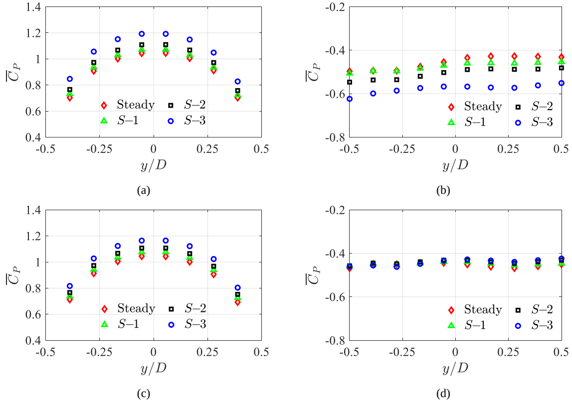
Figure 15. Mean pressure coefficients in Sinusoidal -type inflows: (a) and (b) windward and leeward sides during a_p ramp-up; (c) and (d) during a_p ramp-down.
