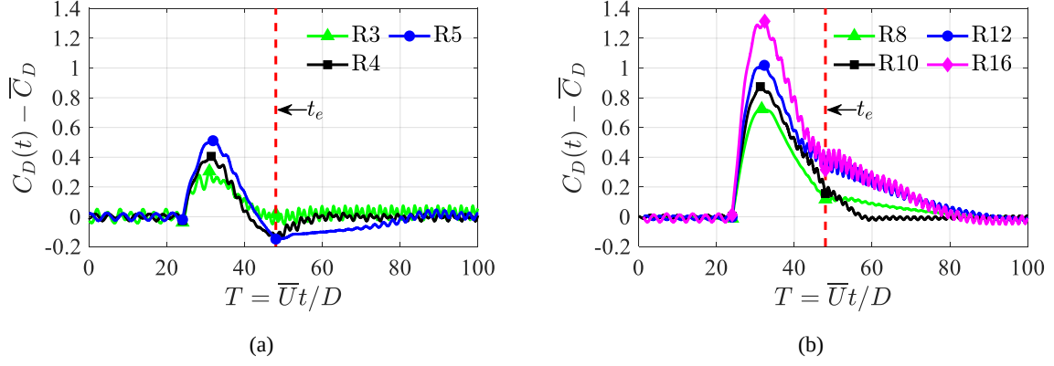
Figure 21. Drag coefficients for different rectangular cylinders for Sinusoidal -type inflow S -3: (a) R 3, R 4, R 5; (b) R 8, R 10, R 12 and R 16;
