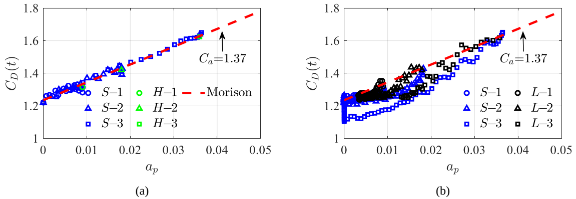
Figure 14. Instantaneous drag coefficients of R4 vs a_p : (a) ramp-up; (b) ramp-down.
