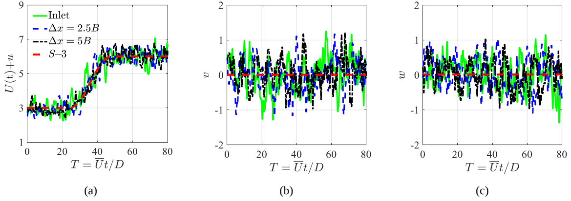
Figure 9. Time history of wind speed for Turbulent -type accelerating inflow: (a) U(t)+u ; (b) v ; (c) w .
