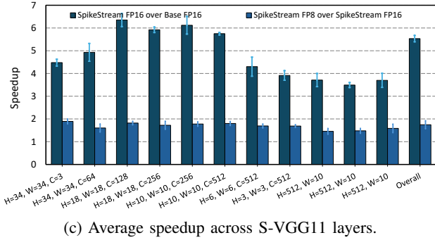
Fig. 3: Performance and memory footprint evaluation on S-VGG11, showing average values and standard deviations for a batch size of 128 input frames.
