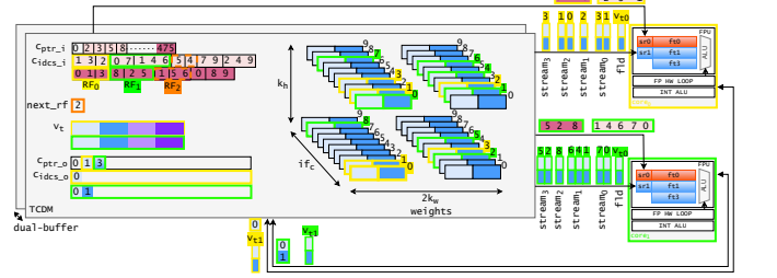
(b) SpikeStream dataflow assuming k_h = k_w = \text{stride} = 2 , 2 worker cores and FP32 weights.
