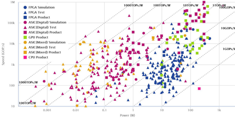
Fig. 2. Overview on state-of-the-art Neural Network accelerators based on available data collected in [76]. Legenda: Simulation means GOPS/W values collected from post-layout simulation; Test means from prototype devices; Product means from off-the-shelf devices.
