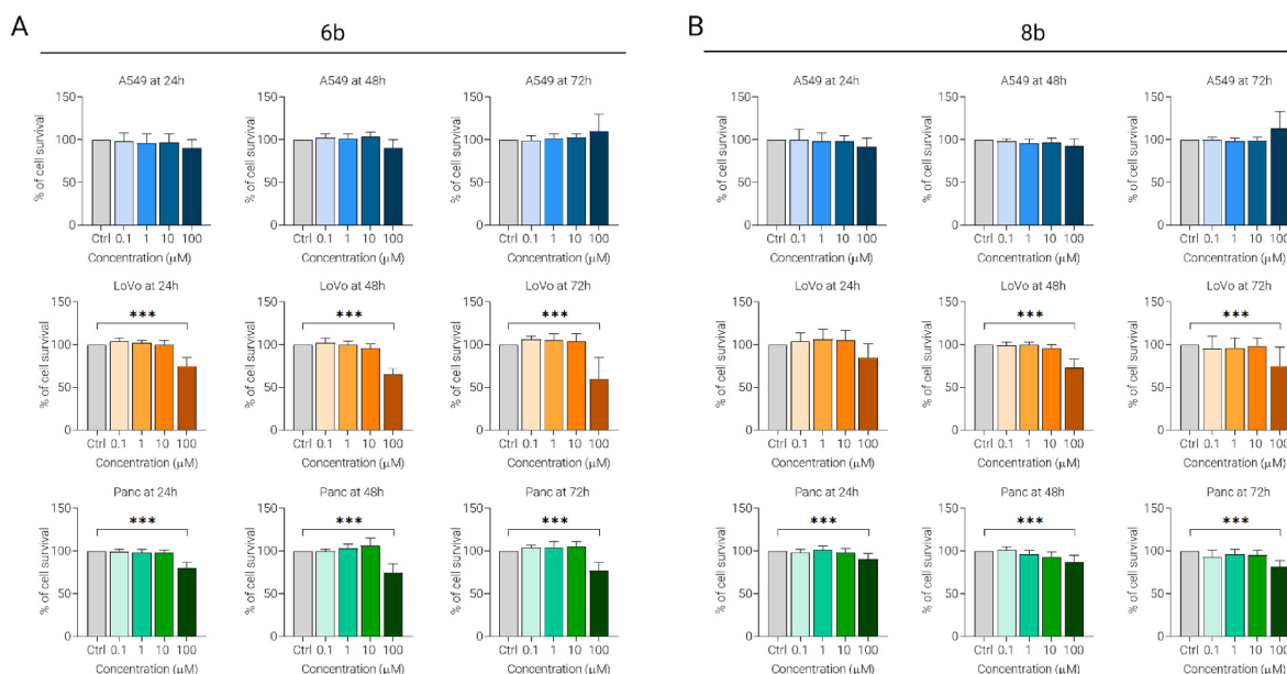
Fig. 10. Cytotoxicity evaluation (expressed as % of cell survival) for compounds 6b (A) and 8b (B) against A549, LoVo and Panc-1 cancer cell lines. Cell survival was evaluated at 0.1, 1, 10, 100 \mu M at 24, 48, 72 h after exposure. Data are reported as mean \pm SD. *** = p < 0.0001 .
