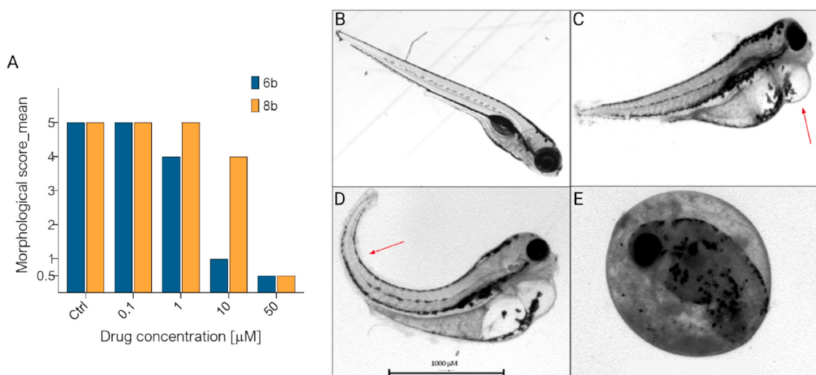
Fig. 11. Morphological score (A) obtained from the average values of the sample score sheet (Tables SI-X) and representative body shape morphology of zebrafishes observed during treatment with high dose of compounds 6b and 8b : normal body shape (B); abnormal heart morphology: heart severely enlarged (C); abnormal body shape: severely curved tail (D); abnormal development: embryo died before complete development (E). The main morphological alteration observed are pointed with a red arrow. Exposure time: 120 h, 5 days-post-fertilization.
