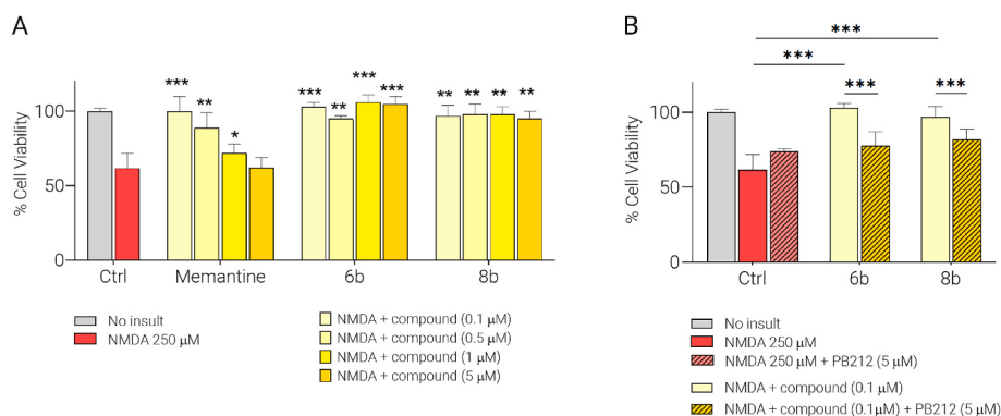
Fig. 8. (A) Neuroprotective effect expressed as % of cell viability (SHSY5Y cells) of compounds 6b , 8b and memantine (used as reference drug) at four concentration (0.1–5 \mu M) against 250 \mu M NMDA-induced cytotoxicity in SH-SY5Y neuroblastoma cells. (B) Neuroprotective effect of compounds 6b and 8b (0.1 \mu M) in the presence of NMDA (250 \mu M) and a combination of NMDA and PB212 (5 \mu M). Cell viability was assessed by MTT test. Each bar represents the mean \pm SD of three independent experiments; * p < 0,1; ** p < 0,01; *** p < 0,001.
