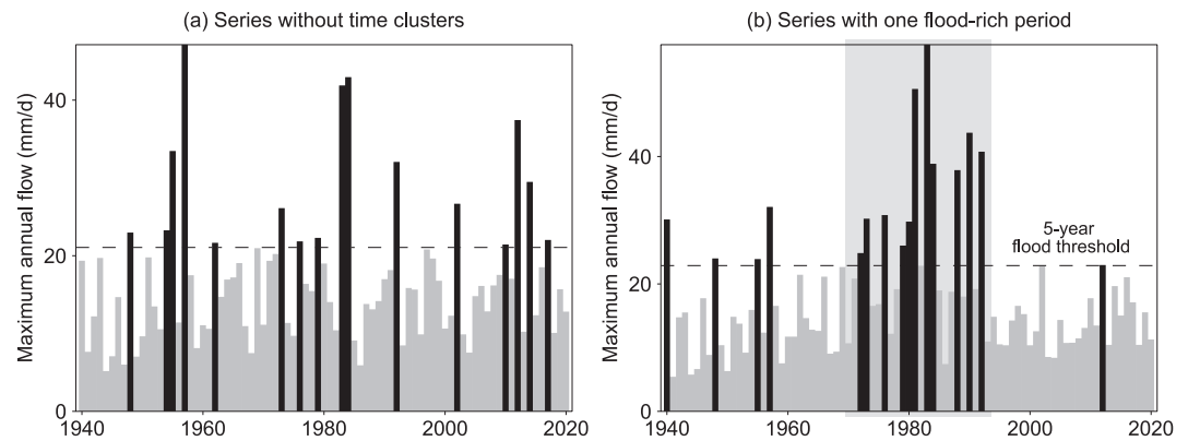
Figure 2. Example of a flood time series (a) without significant time clusters (gauge ID 83690000) and (b) with a significant flood-rich period ( p < 0.001 ) (gauge ID 83440000). The dashed line is the 5-year return period threshold, black bars are flows above the threshold and gray bars are flows below the threshold. The shaded area in (b) shows the window when the flood-rich period was detected.
