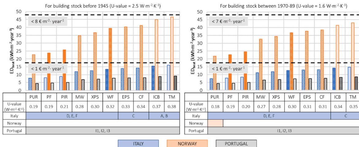
Fig. 2. Energy demand for heating when a 100 mm thickness of each thermal insulation material is applied to external walls in Italy, Norway, and Portugal [34]: a) initial U-value of 2.5 \text{ W}\cdot\text{m}^{-2}\cdot\text{K}^{-1} corresponding to the highest U-value for buildings before 1945 [35]; b) initial U-value of 1.6 \text{ W}\cdot\text{m}^{-2}\cdot\text{K}^{-1} corresponding to the highest U-value for buildings between 1970 and 1989 [35].
