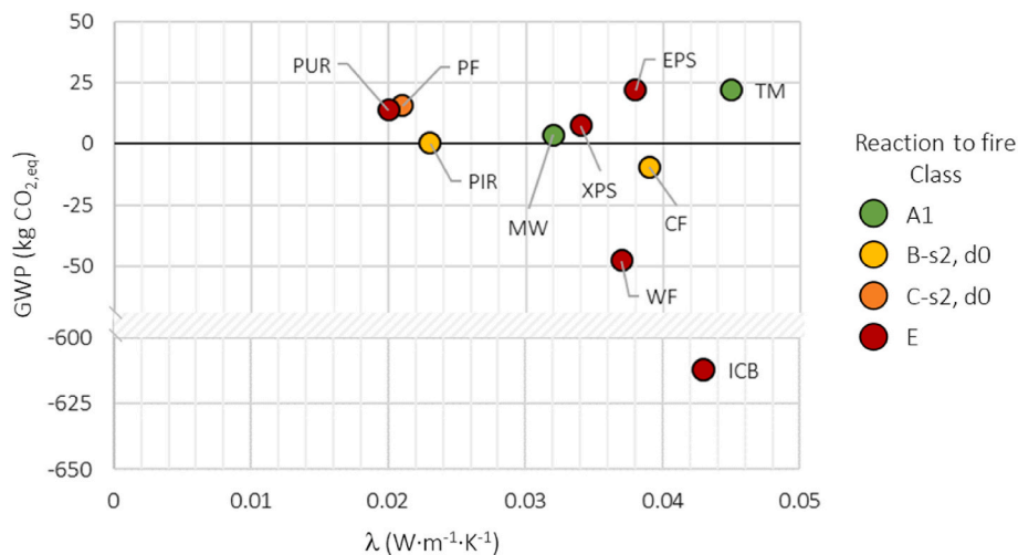
Fig. 3. Total Global Warming Potential (GWP) versus thermal conductivity ( \lambda ), dots are coloured based on the reaction to fire class.
