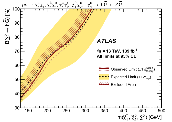
Fig. 6. Observed and expected 95% CL limits on the pure-higgsino branching fraction to B(\tilde{\chi}_1^0 \rightarrow h\tilde{G}) as a function of the higgsino mass m(\tilde{\chi}_1^0) assuming it decays via either \tilde{\chi}_1^0 \rightarrow h\tilde{G} or \tilde{\chi}_1^0 \rightarrow Z\tilde{G} . Limits are obtained by performing a statistical combination of the three signal regions SR1h, SR1Z and SR2. The \pm 1\sigma variation on the expected limit is shown. The dotted lines indicate the observed limit obtained by a variation of theoretical prediction for the neutralino production cross-section by \pm 1\sigma . Values of B(\tilde{\chi}_1^0 \rightarrow h\tilde{G}) larger than the observed 95% CL limit are excluded, as indicated by the hatched area.
