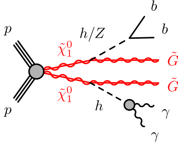
Fig. 1. The diagram shows the topology considered by this search, the production of two neutralinos \tilde{\chi}_1^0 , which decay into a gravitino \tilde{G} and either a Higgs boson h or a Z boson. The search aims to select events in which a pair of photons is produced by a Higgs boson from one \tilde{\chi}_1^0 , while a pair of b -quarks is produced by either the decay of a Higgs boson or a Z boson from the other.
