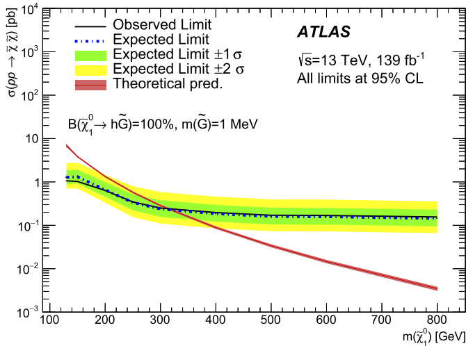
Fig. 5. Observed and expected limits on the pure higgsino cross-section at 95% CL assuming B(\tilde{\chi}_1^0 \rightarrow h\tilde{G}) = 100\% for different \tilde{\chi}_1^0 masses, obtained by a statistical combination of the three signal regions SR1h, SR1Z and SR2. The inner and outer bands indicate the 1\sigma and 2\sigma variation on the expected limit respectively.
