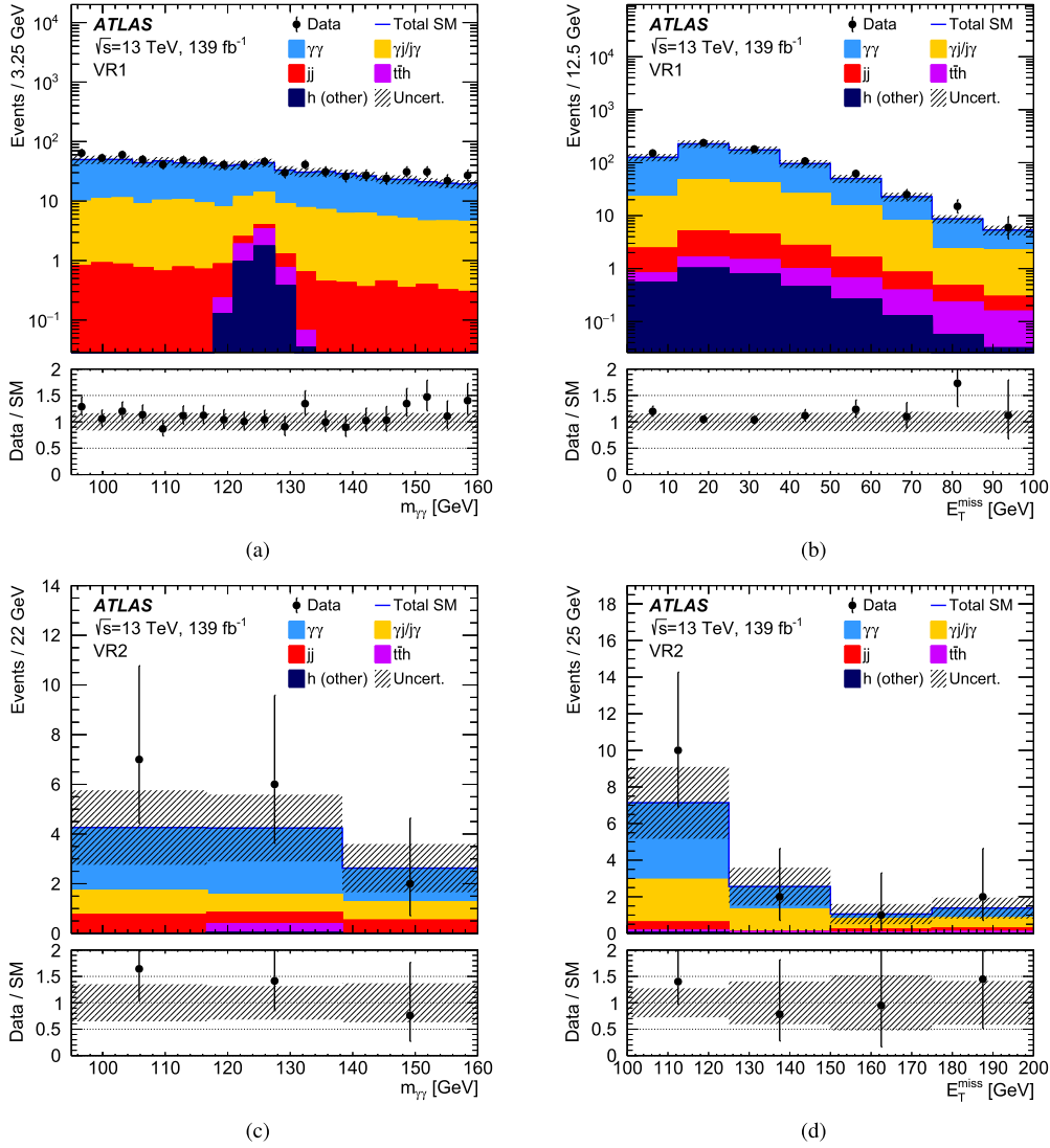
Fig. 3. Distribution of the diphoton invariant mass in both validation regions: (a) VR1 and (c) VR2 as well as the missing transverse momentum in both validation regions: (b) VR1 and (d) VR2. The solid histograms are stacked to show the SM expectations after the 2×2D background estimation technique is applied. Background and signal predictions are normalised to the luminosity. The background category ‘ h (other)’ includes events originating from VBF, Vh , ggF , thq , thW and b\bar{b}h , all subdominant in this signature. Statistical and systematic uncertainties are indicated by the shaded area. The lower panel of each plot shows the ratio of the data to the SM prediction for the respective bin. The first and last bins include the underflows and overflows respectively.
