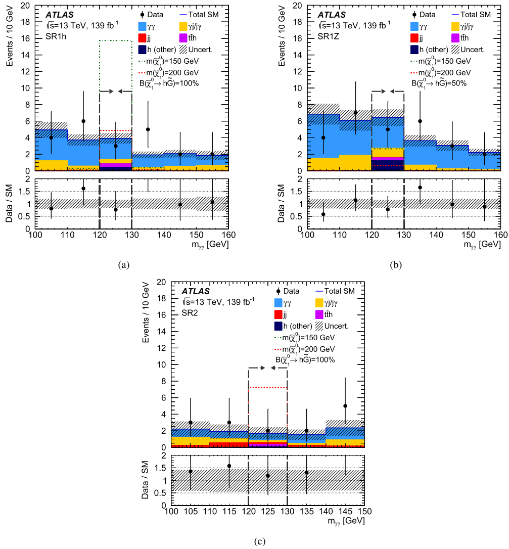
Fig. 4. Distribution of the diphoton invariant mass with all selections of the signal regions applied, except on m_{\gamma\gamma} itself, for the three signal regions: (a) SR1h, (b) SR1Z and (c) SR2. The background estimation techniques described in the text are applied. The different backgrounds are stacked to add up to the total SM prediction in each bin. The predicted yields for signal benchmark models of varying \tilde{\chi}_1^0 mass are also overlaid (not stacked) assuming B(\tilde{\chi}_1^0 \rightarrow h\tilde{G}) to equal (a) 100%, (b) 50% and (c) 100%. Background and signal predictions are normalised to the luminosity. The background category ‘h (other)’ includes events originating from VBF, Vh , ggF , thq , thW and b\bar{b}h , all subdominant in this signature. The sizes of the statistical and systematic uncertainties are indicated by the shaded areas. The lower panels show the ratio of the data to the SM prediction. Arrows indicate the borders of the signal region ( |m_{\gamma\gamma} - 125 \text{ GeV}| < 5 \text{ GeV} ). The first and last bins include the underflows and overflows respectively.
