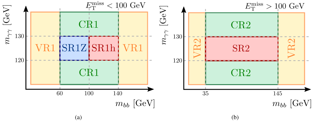
Fig. 2. Schematic overview of the event categorisation. Events with (a) low- E_T^{\text{miss}} and (b) high- E_T^{\text{miss}} are treated separately, while the invariant masses of the photons m_{\gamma\gamma} and b -jets m_{bb} are used to categorise events. The resulting control regions (CR) are used to estimate backgrounds. This estimation is applied to both the validation regions (VR) and the signal regions (SR).
