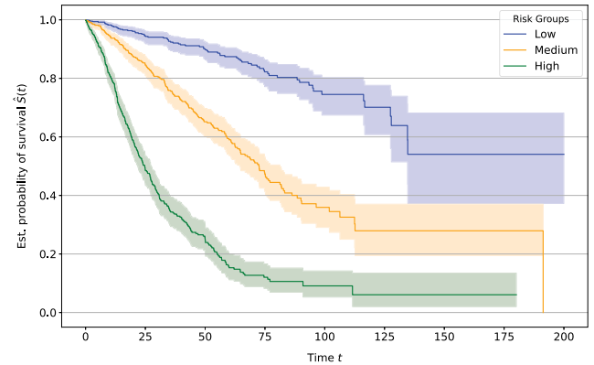
Fig. 2. Kaplan-Meier curves stratified by risk groups based on percentiles.
