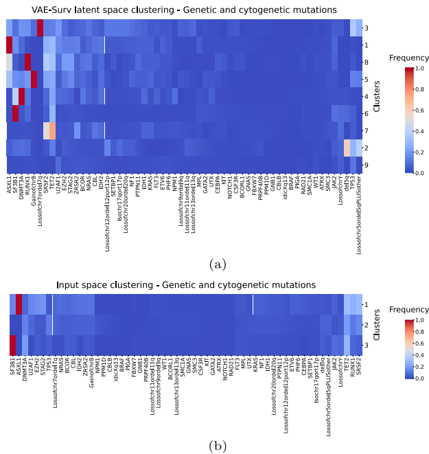
Fig. 6. Clustermaps displaying the frequency of gene mutations and cytogenetic alterations within each identified cluster. The color intensity corresponds to the prevalence of each genetic feature in the clusters, providing insights into their mutational landscape. Panels (a) and (b) show the results from clustering on the VAE latent space and on the input space, respectively.
