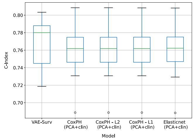
Fig. 3. Comparison of VAE-Surv and CoxPH models using PCA-reduced genetic features and clinical covariates.
