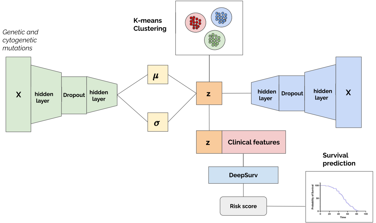
Fig. 1. Schematic representation of the VAE-Surv computational framework. Genetic and cytogenetic markers are treated as binary input vectors of a Variational Autoencoder (VAE) for dimensionality reduction. The latent feature space, obtained by the VAE, is concatenated with clinical variables to form an enriched feature set. This combined feature set is then exploited by a deep learning generalization of the Cox proportional hazards (DeepSurv [22]) model for survival risk prediction. The dimensionality of the latent space z is optimized as a hyperparameter of the framework.
