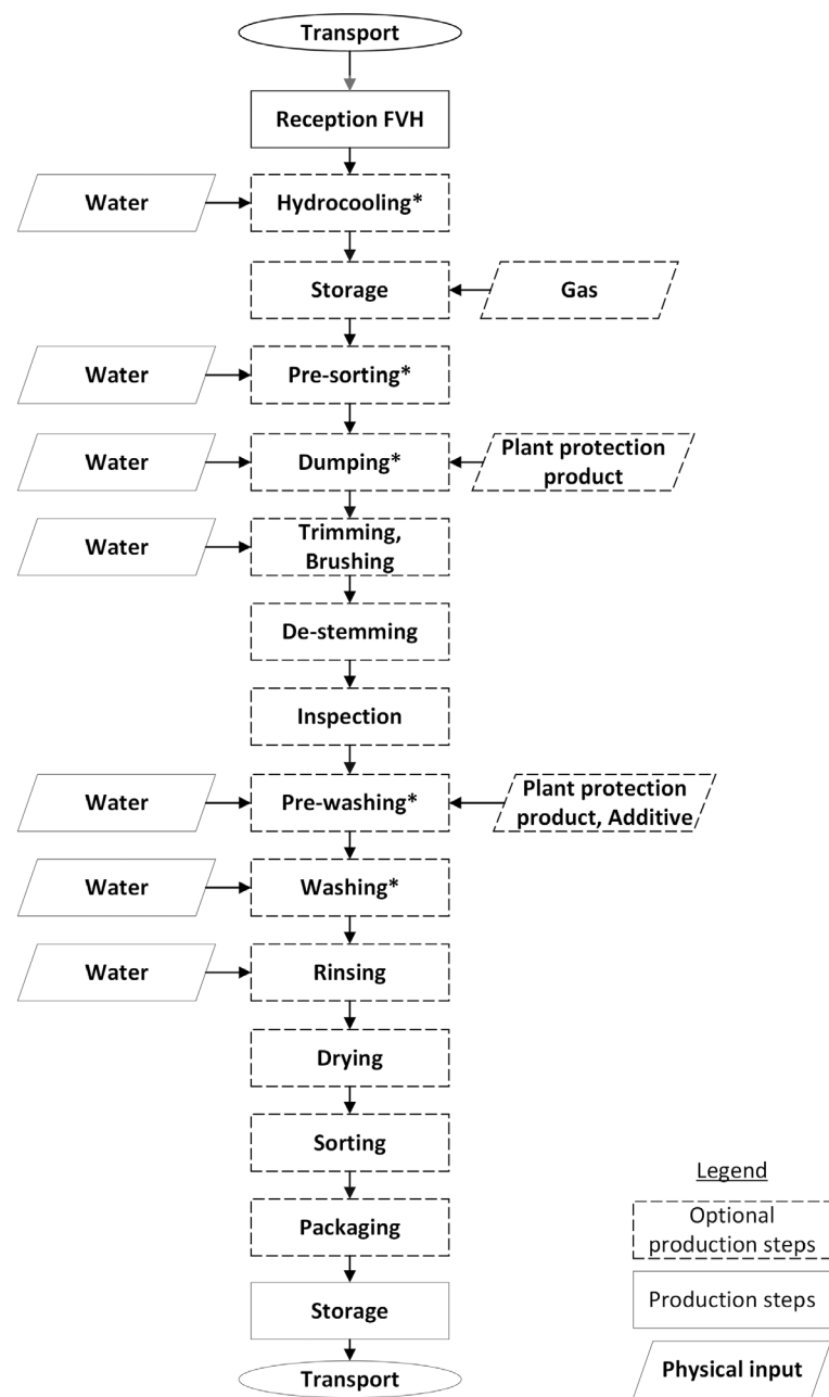
FIGURE 2 A general flow chart for handling and processing fresh-whole fruits, vegetables and herbs (FVH), which includes steps where water can be used. The flow chart can vary between FBOps (e.g. following order of steps, optional steps present or not) and represents a general description of the post-harvest processing and handling operations. *Production steps sampled during EFSA's outsourced activities (Gil et al., 2025).
