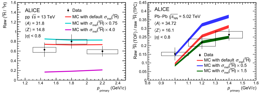
Fig. 1. Left: raw primary {}^3\text{H}/{}^3\text{H} ratio as a function of the momentum p_{\text{primary}} in pp collisions at \sqrt{s} = 13 TeV. Right: ratio between the raw number of {}^3\text{H} candidates reconstructed in the TOF and the raw number of {}^3\text{H} reconstructed in the TPC in Pb-Pb collisions at \sqrt{s_{\text{NN}}} = 5.02 TeV as a function of the momentum p_{\text{primary}} . In both panels, data are shown in black, the statistical and systematic uncertainties are shown as vertical bars and boxes, respectively. The results from ALICE MC simulations based on GEANT4 are shown as coloured bands, the different colours referring to the different inelastic cross sections implemented in the simulations, with default \sigma_{\text{inel}} described in Ref. [56]. The width of the MC band represents the statistical uncertainty of the simulation.
