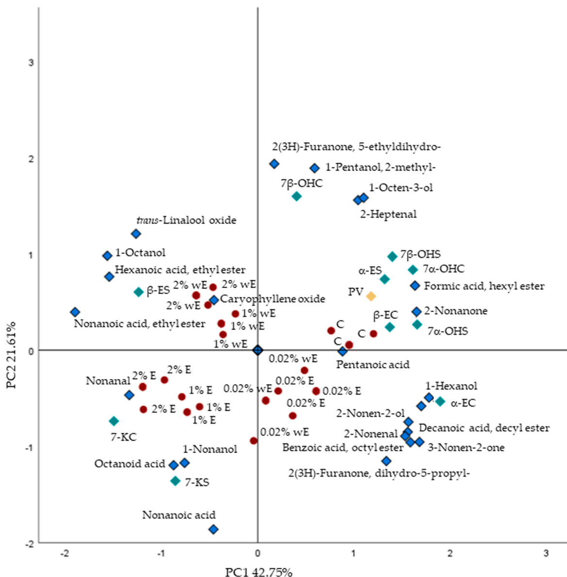
Fig. 4. Principal component analysis Bi-Plot of VOCs and POPs. 7 \alpha -OHS, 7 \alpha -hydroxysitosterol; 7 \beta -OHS, 7 \beta -hydroxysitosterol; 7 \alpha -OHC, 7 \alpha -hydroxycampesterol; 7 \beta -OHC, 7 \beta -hydroxycampesterol; 7-KS, 7-ketositosterol; 7-KC, 7-ketocampesterol; \alpha -ES, \alpha -epoxysitosterol; \beta -ES, \beta -epoxysitosterol; \alpha -EC, \alpha -epoxycampesterol; \beta -EC, \beta -epoxycampesterol.
