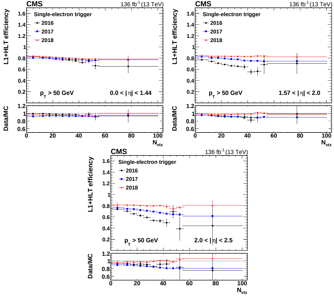
Figure 10. The L1+HLT efficiency of the single-electron HLT path with p_T > 27 (32) GeV in 2016 (2017 and 2018) with respect to an offline-reconstructed electron as a function of N_{\text{vtx}} , obtained for 0 < |\eta| < 1.44 (upper left), 1.57 < |\eta| < 2.0 (upper right), and 2.0 < |\eta| < 2.5 (lower). The electron p_T is required to be above 50 GeV. The lower panel of each plot shows the ratio of data to MC simulation. The vertical bars on the markers represent combined statistical and systematic uncertainties.
