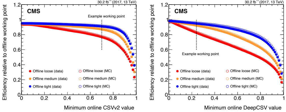
Figure 23. Efficiency of jets b tagged offline to pass the online CSVv2 (left) and DeepCSV (right) b tagging requirement, as a function of the online requirement. Three offline selections are shown: Loose (red), Medium (orange), and Tight (blue). Data are shown in closed circles; the result of the simulation is shown in open circles. The right plot is obtained using 2017 data and MC simulation but using the DeepCSV algorithm as it was run in 2018.
