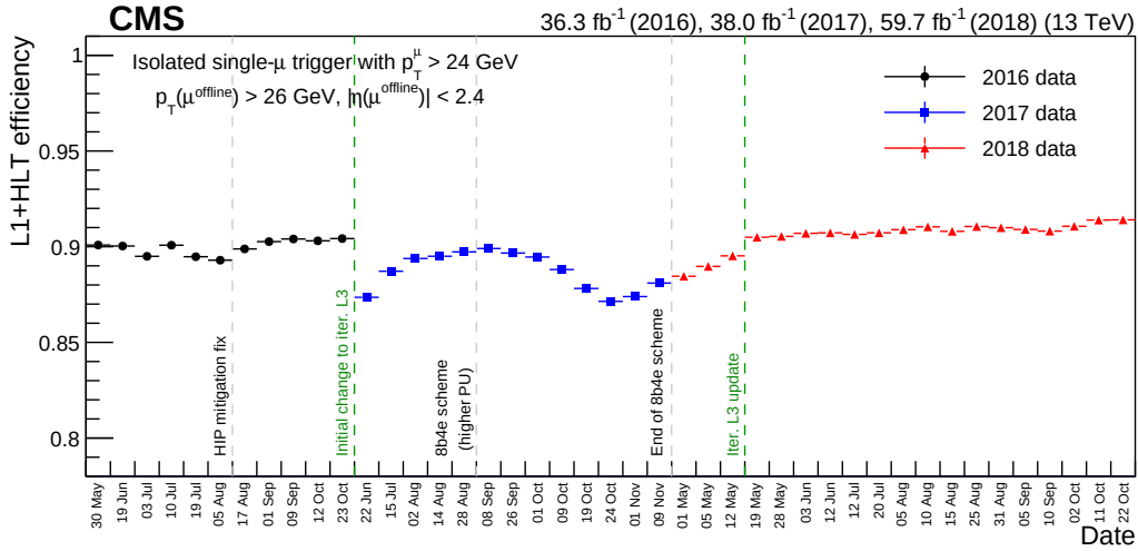
Figure 6. Evolution of the isolated single-muon trigger efficiency with p_T > 24 GeV as a function of data-taking dates during the Run 2 period from 2016 to 2018. Each point is the efficiency measured using the data with an integrated luminosity of about 3 \text{ fb}^{-1} . Dashed lines show the changes in the LHC or CMS conditions that could have an impact on the trigger performance, such as the fix for the degradation of the inner tracker as a result of heavily ionizing particles (“HIP mitigation fix”) or the change in the filling scheme for pp collisions at the LHC (“8b4e scheme”) that led to higher PU in CMS until the end of 2017. The change of the reconstruction algorithm for L3 muons are presented as green dotted lines, including the replacement of cascade or tracker muon algorithm to the iterative algorithm (“Change to iter. L3”) and the update of the iterative algorithm to overcome the limitations observed in 2017 (“Iter. L3 update”).
