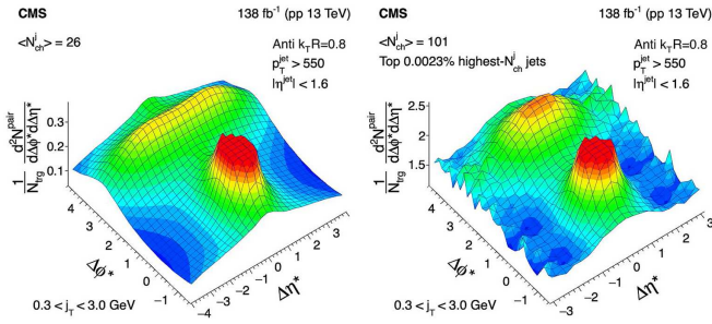
FIG. 2. Results for 2D two-particle angular correlation functions for particle 0.3 < j_T < 3.0 GeV from inclusive (left) and the highest (right) N_{\text{ch}}^j jets, for anti- k_T R = 0.8 algorithm with p_T^{\text{jet}} > 550 GeV and |\eta^{\text{jet}}| < 1.6 .
