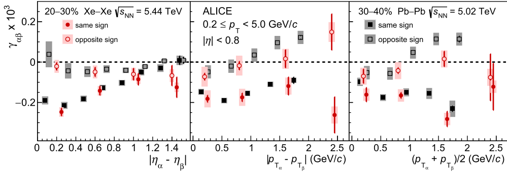
Fig. 2. The dependence of \gamma_{\alpha\beta} on the pseudorapidity difference |\eta_\alpha - \eta_\beta| (left panel), the transverse momentum difference |p_{T\alpha} - p_{T\beta}| (middle panel), and the average transverse momentum (p_{T\alpha} + p_{T\beta})/2 (right panel) for pairs of particles with same (closed markers) and opposite (open markers) charges from 20–30% Xe-Xe collisions at \sqrt{s_{NN}} = 5.44 TeV (red circles) compared to results from 30–40% Pb-Pb collisions at \sqrt{s_{NN}} = 5.02 TeV (black squares) [42]. The Pb-Pb and Xe-Xe same-charge points are slightly shifted along the horizontal axis for better visibility in all panels. Bars (boxes) denote statistical (systematic) uncertainties.
