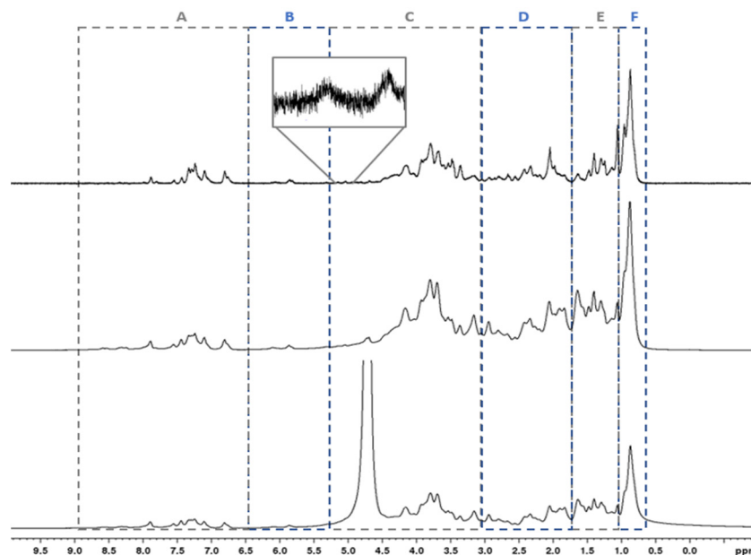
Figure 2. ^1\text{H} NMR spectra of microalgae-based product MR in \text{D}_2\text{O} (298K @ 600 MHz). From bottom to top, spectra acquired using the pulse sequences: zgcprr , noesypr1d , and cpmgpr1d , respectively. Six typical regions are highlighted by dashed square boxes: (A) aromatic protons from amino acids and nucleobases (9.0–6.5 ppm); (B) nucleobases and double-bond (lipids and carotenoids) protons (6.5–5.3 ppm), the expansion in cpmgpr1d spectrum highlights diacylglycerol methylene group; (C) amino acids, carbohydrates (5.5–3.0 ppm); (D) methylene protons of amino acids/peptides and carboxyl-rich alicyclic molecules (3.0–1.7 ppm); (E) methylene protons of lipids and amino acids/peptides (1.7–1.0 ppm); (F) methyl protons of amino acids and lipids.
